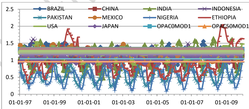
Fig 2. Angstrom Exponent ( \alpha ) plot for OPAC WASO Model 1 Angstrom Exponent ( \alpha ) and MERRA averaged Angstrom Exponent ( \alpha ) for ten countries (Nigeria, Ethiopia, Brazil, USA, Pakistan, Mexico, Japan, China, Indonesia and India)
