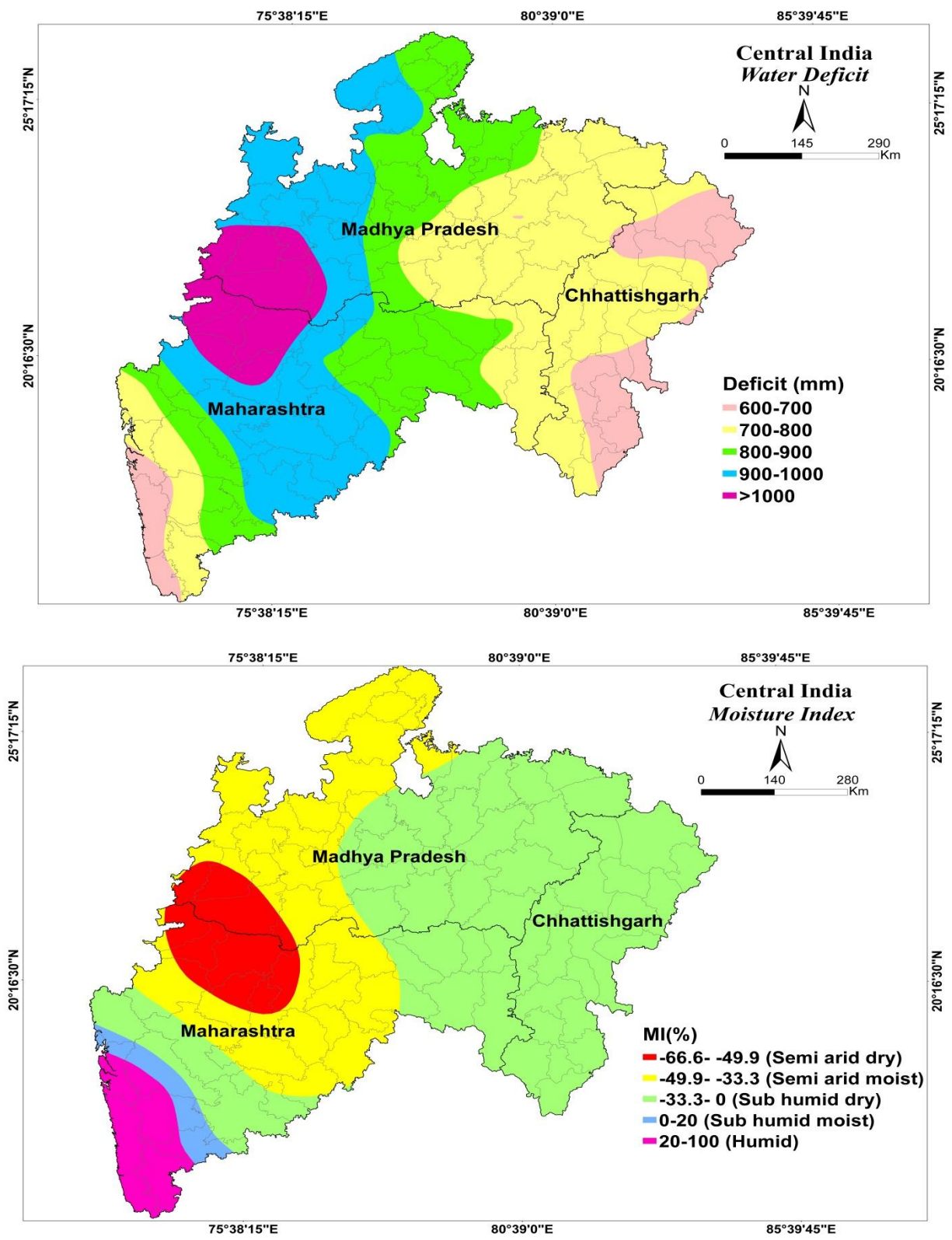
Figure.2: Spatial variability of mean annual Rainfall, Water deficit and Moisture Index of Central India
