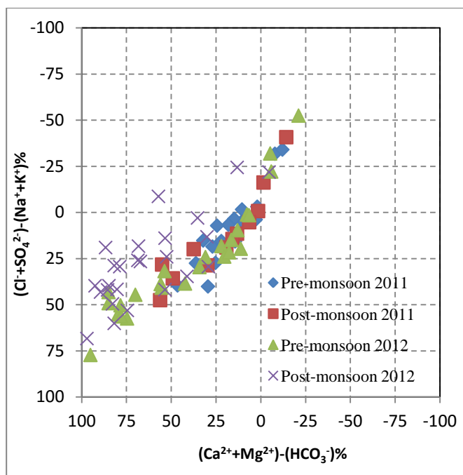
Fig. 5. Langelier and Ludwig plot (modified).
