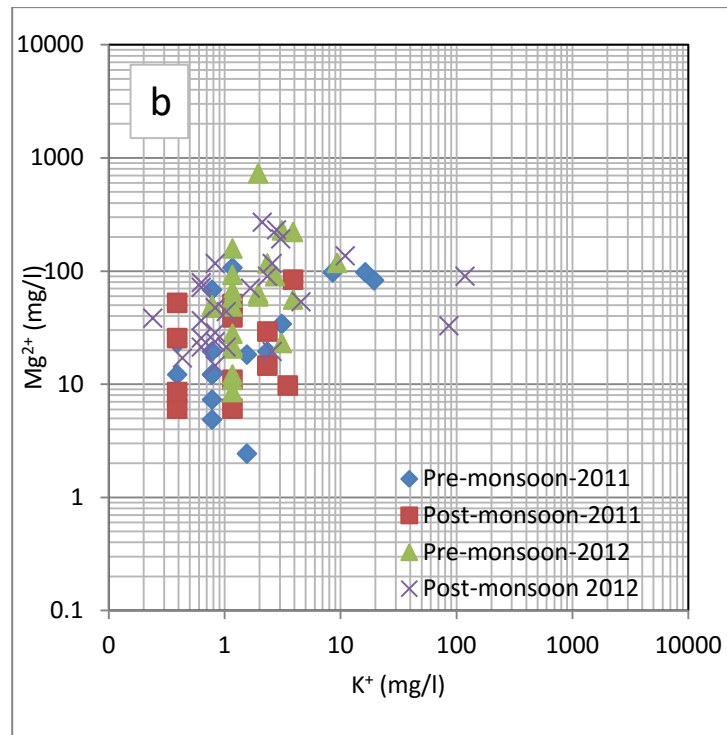
Supplementary Material 2. K^+ vs Mg^{2+} plot for (a) surface water and (b) groundwater.
