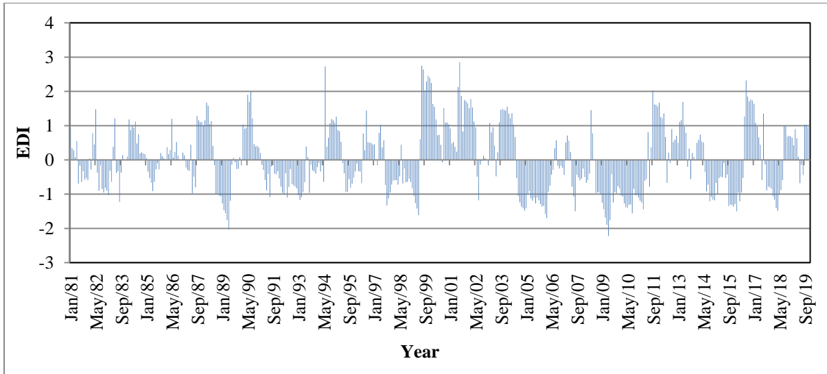
Figure 5: Temporal variation of EDI in Robertsganj block in Sonbhadra district
