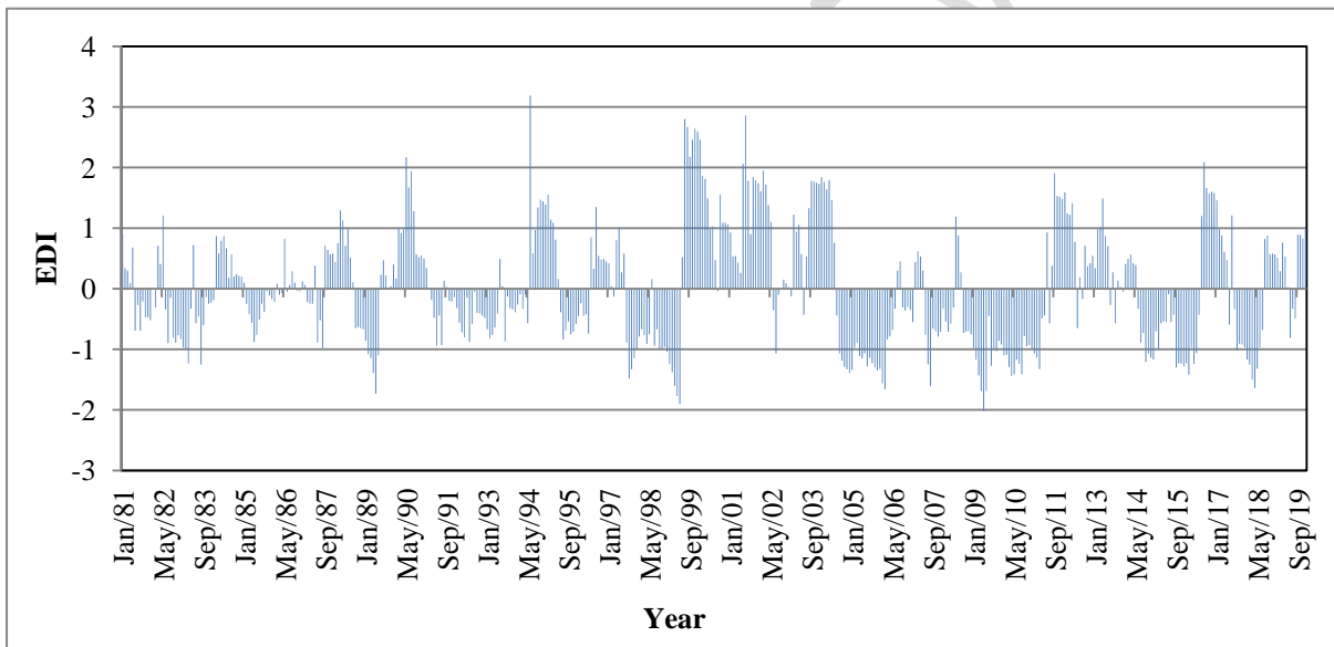
Figure 6: Temporal variation of EDI in Ghorawal block in Sonbhadra district
