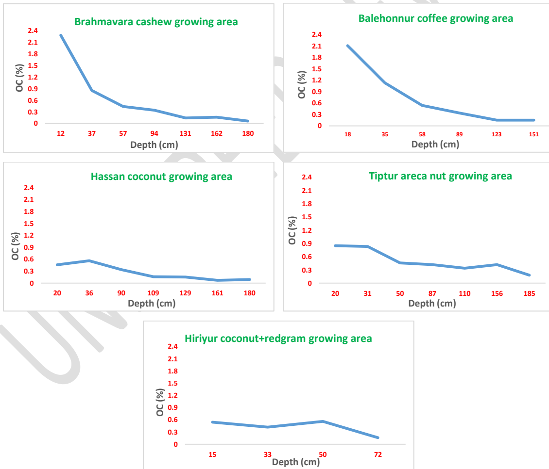
Fig. 2. Depth wise distribution of organic carbon in different pedons
