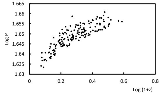
Figure 2: The scatter plot of source observed luminosities against observed redshifts for the extended quasars
