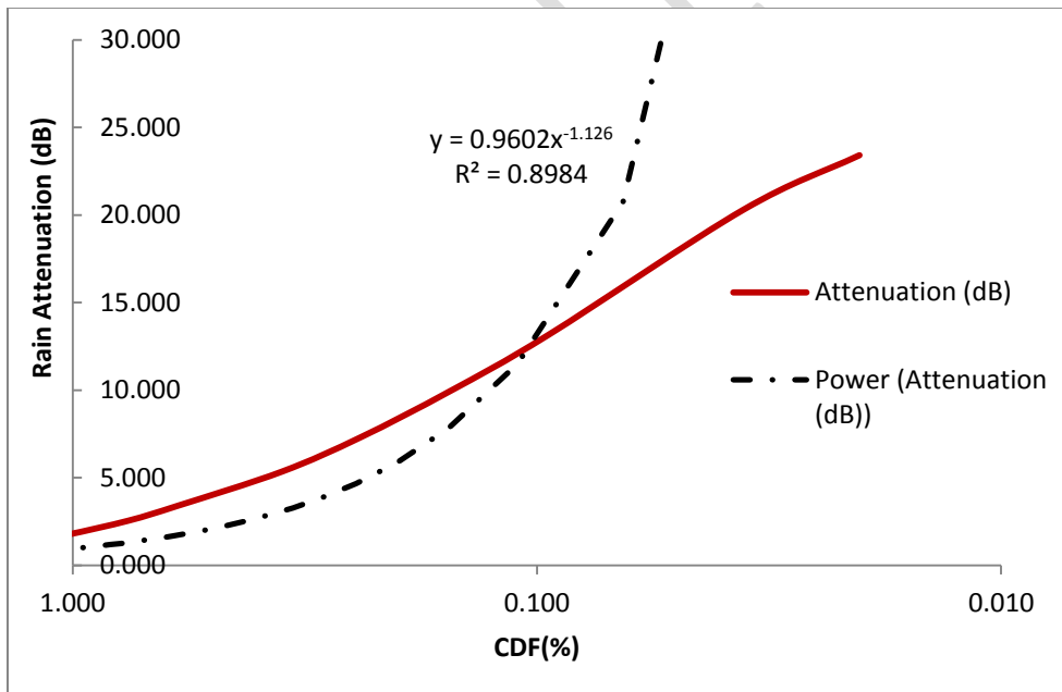
Figure 4: Relationship between CDF and rain attenuation for August 2019.
