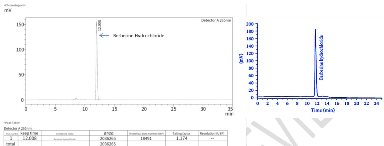
Figure.2. Left side- RP-HPLC chromatogram of sample berberine hydrochloride with retention time 12.008 minute and STD 97% chromatogram on right side with retention time of 11.98 minute
