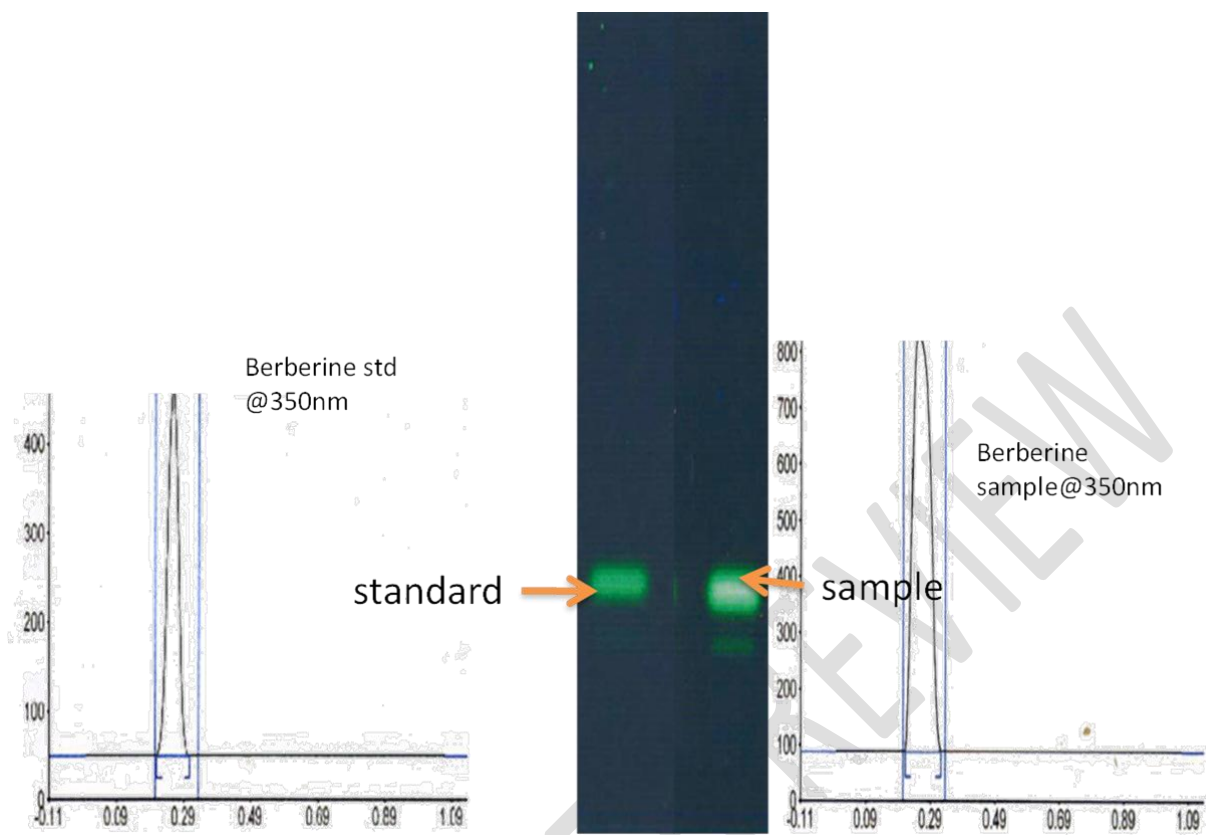
Figure.3. HPTLC quantification of berberine crude with absorption at 350 nm wavelength
