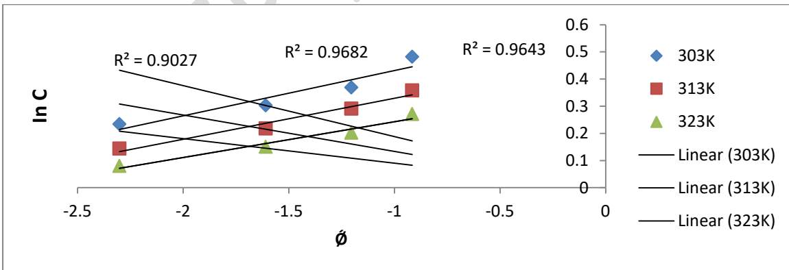
Figure 3: Freundlich Adsorption Isotherm of the Root Extract of Phyllanthus Mellerianus for Mild Steel Surface
