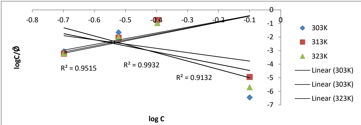
Figure 2: Langmuir Adsorption Isotherm of the Root Extract Phyllanthus Mellerianus for Mild Steel Surface
