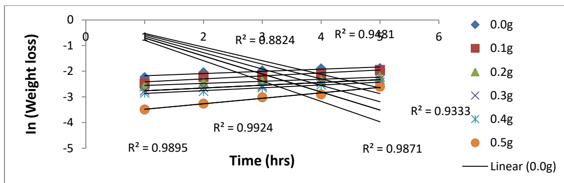
Figure 6. Kinetics analysis of the root extract of Phyllanthus Mellerianus for Inhibitor of Mild Steel Surface
