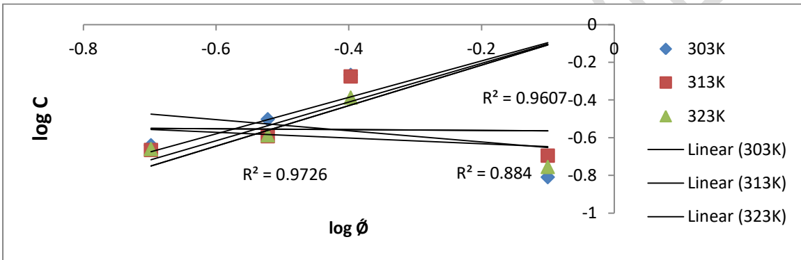
Figure 3: Freundlich Adsorption Isotherm of the Root Extract of Phyllanthus Mellerianus for Mild Steel Surface
