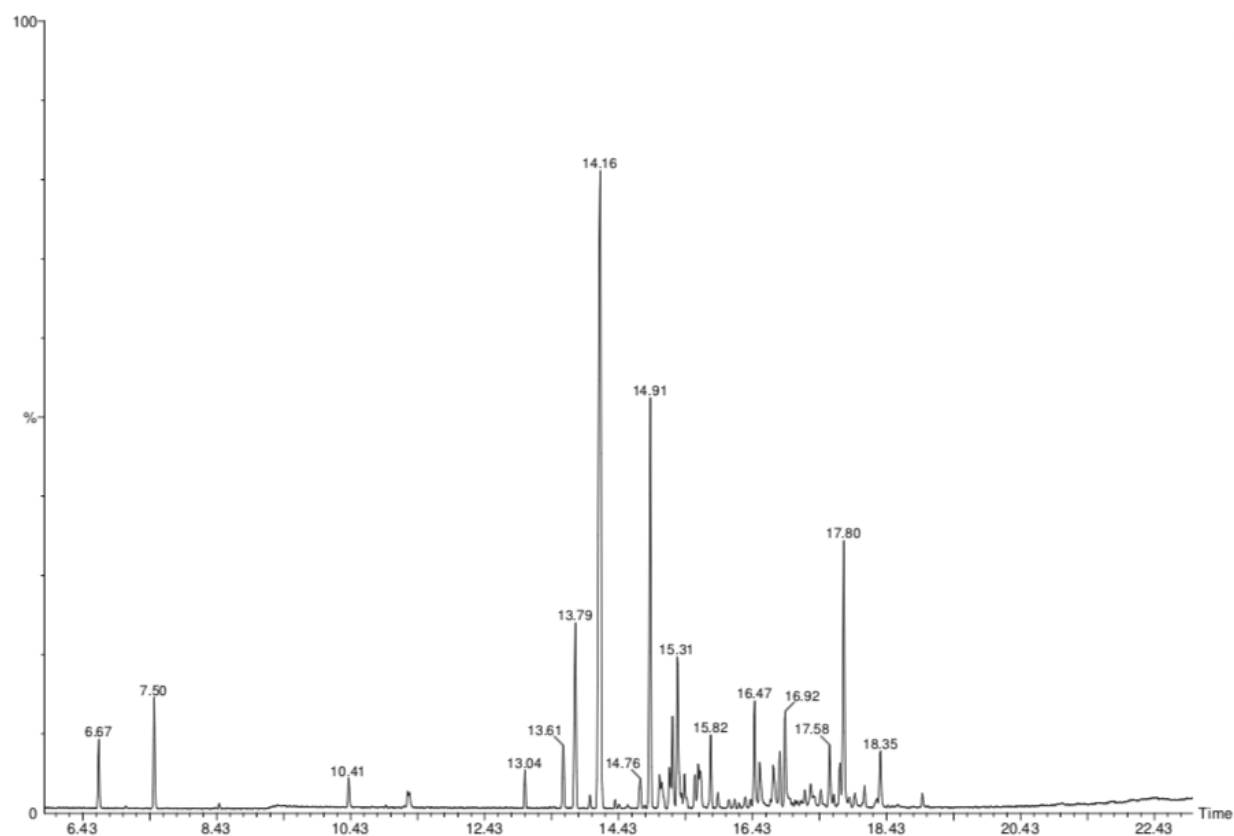
Figure 1: Representative GC-MS chromatogram of Cyperus scariosus essential oil
