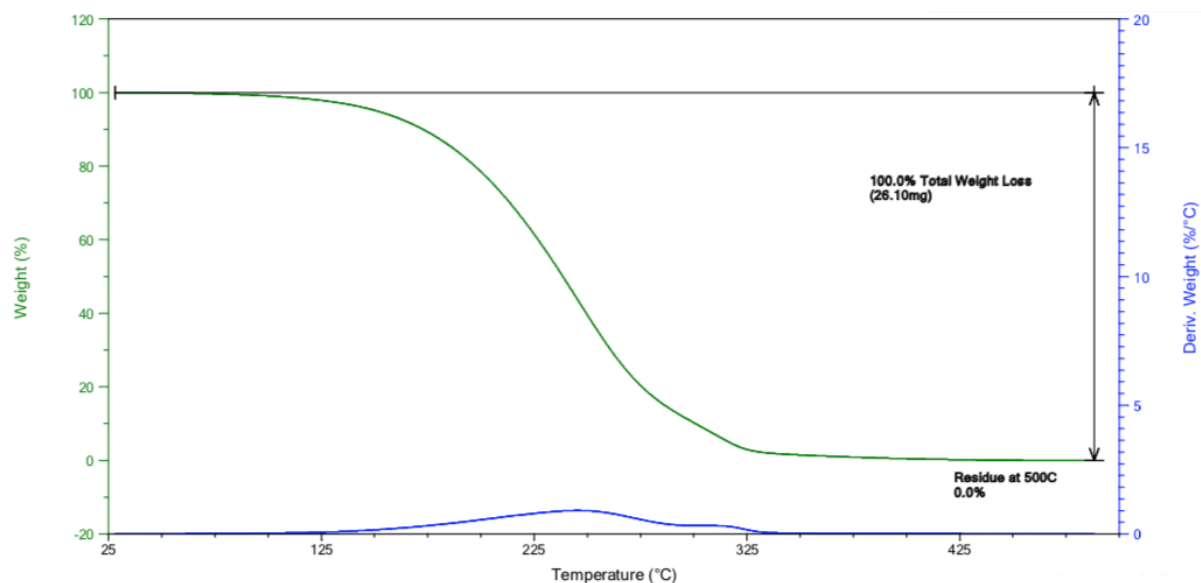
Figure 3: Thermo-gravimetric analysis of Cyperus scariosus essential oil.
