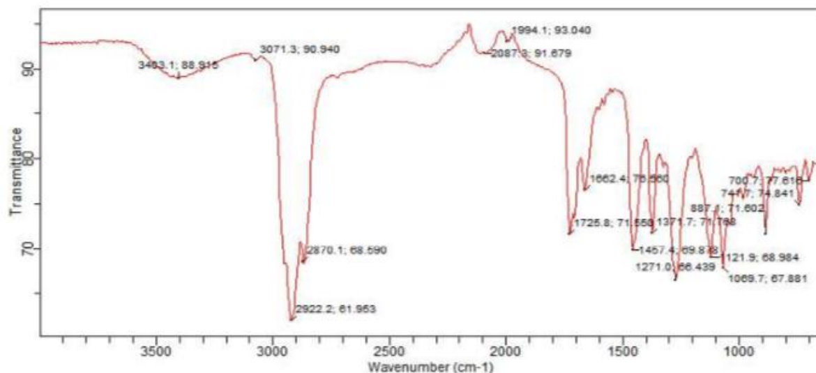
Figure 2: FT-IR analysis of Cyperus scariosus essential oil
