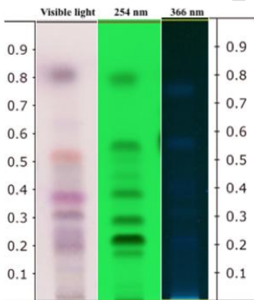
Figure 6: HPTLC fingerprint of Cyperus scariosus essential oil at UV 254, UV 366 and white light after derivatization with vanillin sulfuric acid
