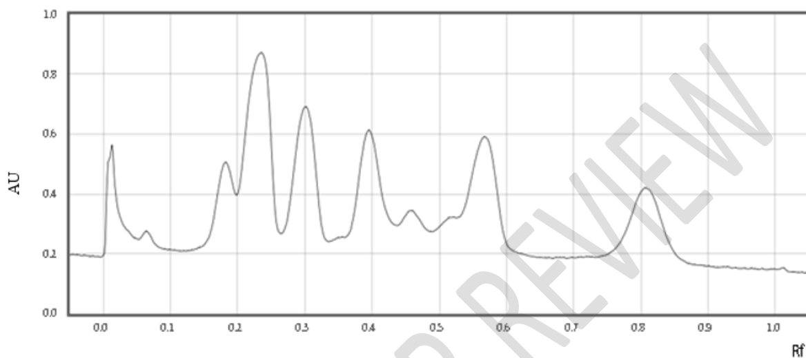
Figure 5: HPTLC peak densitogram profile of Cyperus scariosus essential oil
