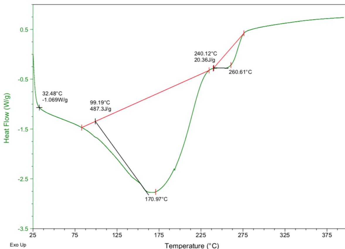
Figure 4: DSC analysis of Cyperus scariosus essential oil
