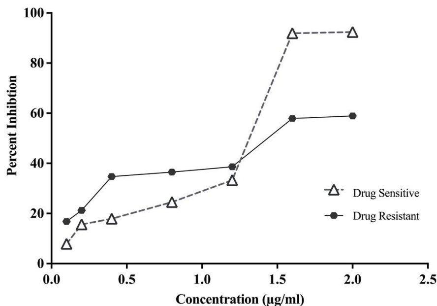
Figure 7: Anti-malarial activity of Cyperus scariosus essential oil
