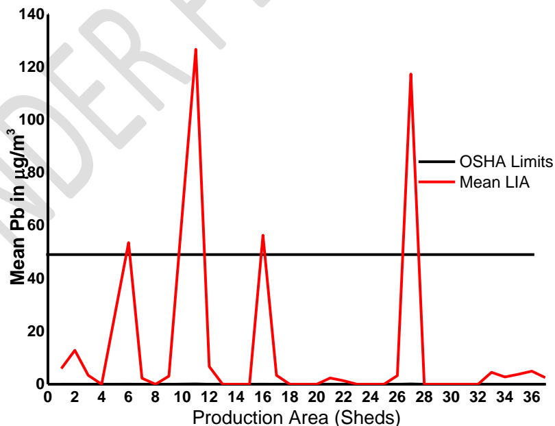
Figure 2: Airborne Lead concentration in production areas (sheds) in the informal sector compared to the USA OSHA limits
