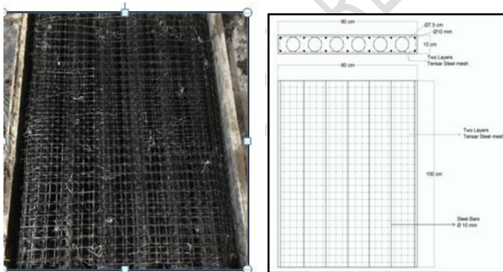
Fig. 9: two layers tenax mesh specimen
