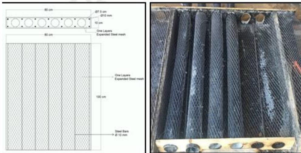
Fig. 6: One layer expanded steel mesh specimen
