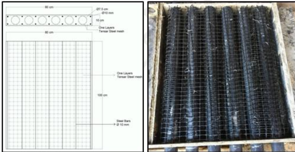
Fig. 8: one layer tenax mesh specimen
