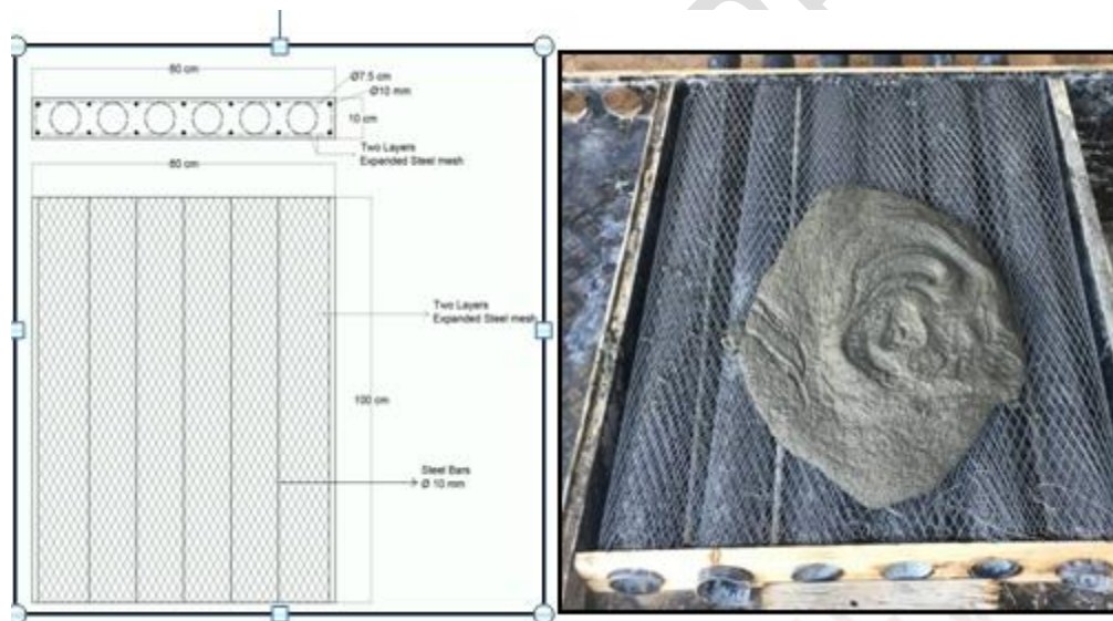
Fig. 7: Two layers expanded steel mesh specimen
