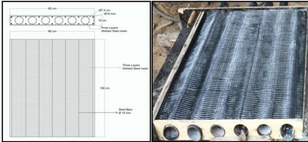
Fig. 4: Three layers welded steel mesh specimen
