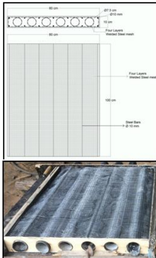
Fig. 5: Four layers welded steel mesh specimen
