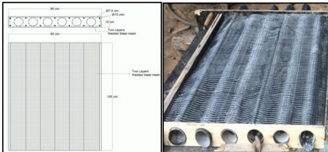
Fig. 3: Two layers welded steel mesh specimen
