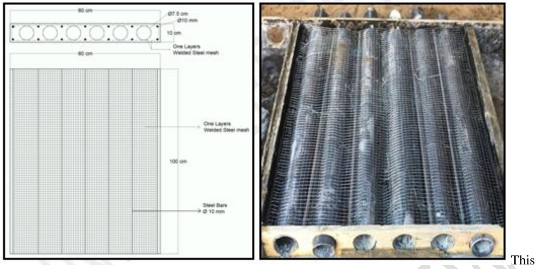
Fig. 2: One layer welded steel mesh specimen
