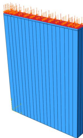
Fig. (27): loading on specimen
