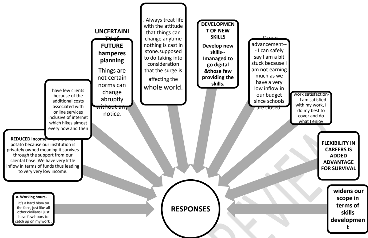
Figure 1. Clusters
