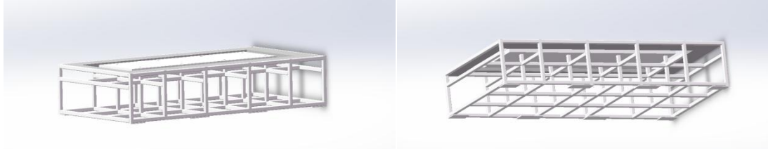
Figure 5 Base frame
