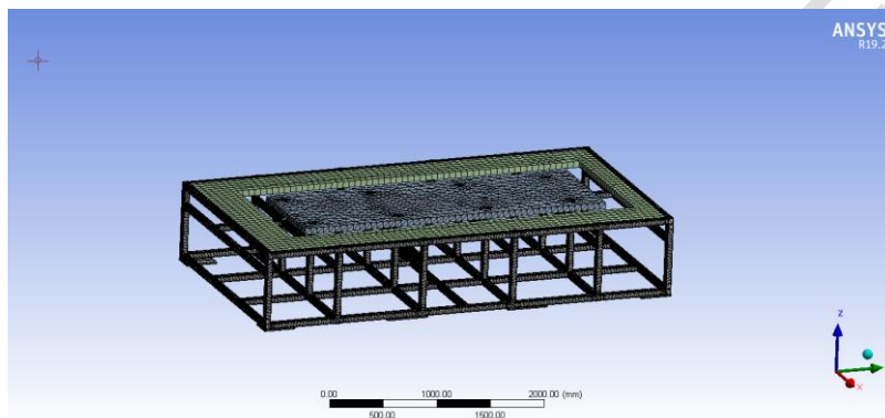
Figure 6 Meshing
