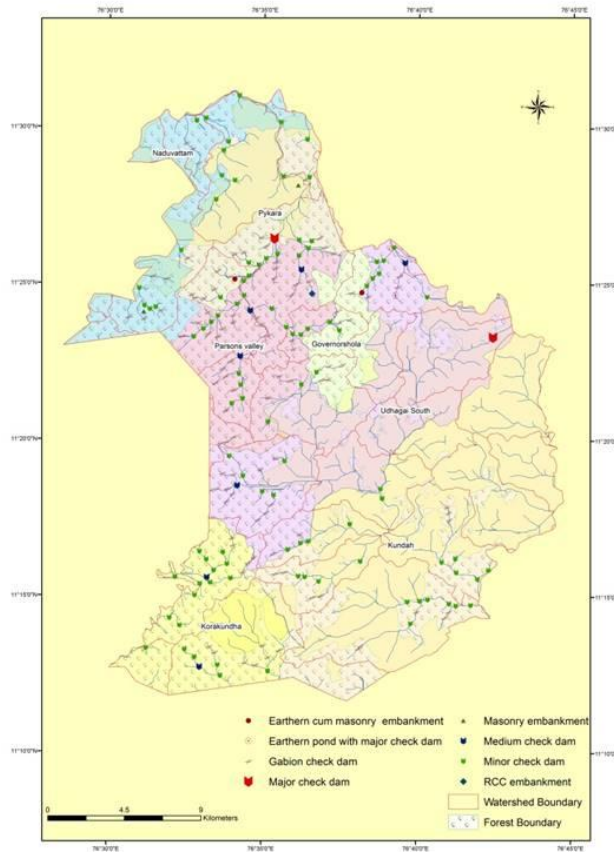
Fig. 9 Location of proposed water management structures in Nilgiris south forest division
