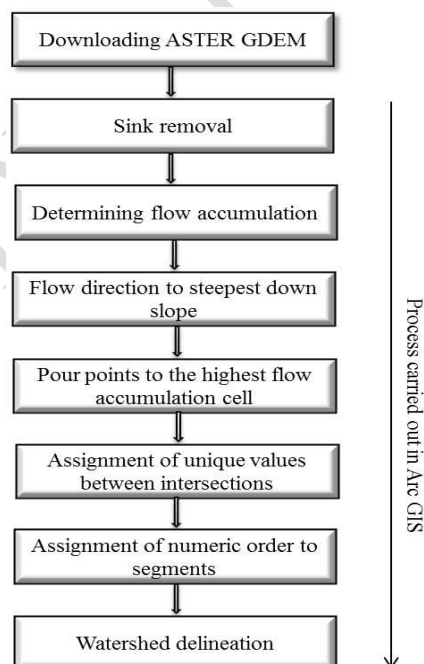
Fig.2. Methodology adopted for delineating watershed and stream feature from ASTER global DEM data.
