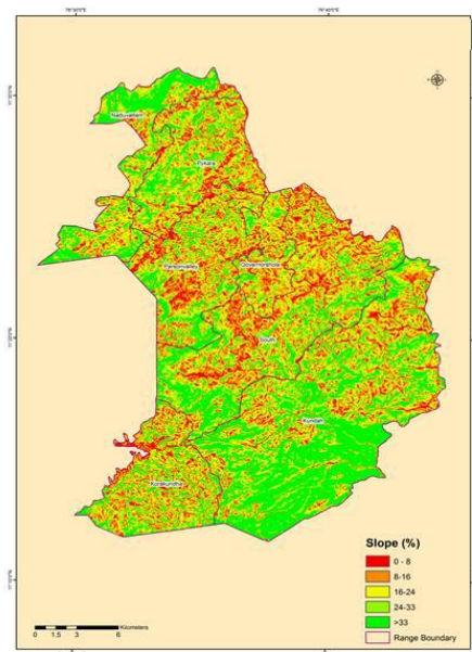
Fig 4. Slope map of Nilgiris south forest division
