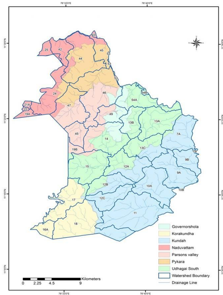
Fig.3 Drainage map of macro watersheds in Nilgiris south forest division
