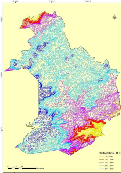
Fig.5 Contour map of Nilgiris south forest division
