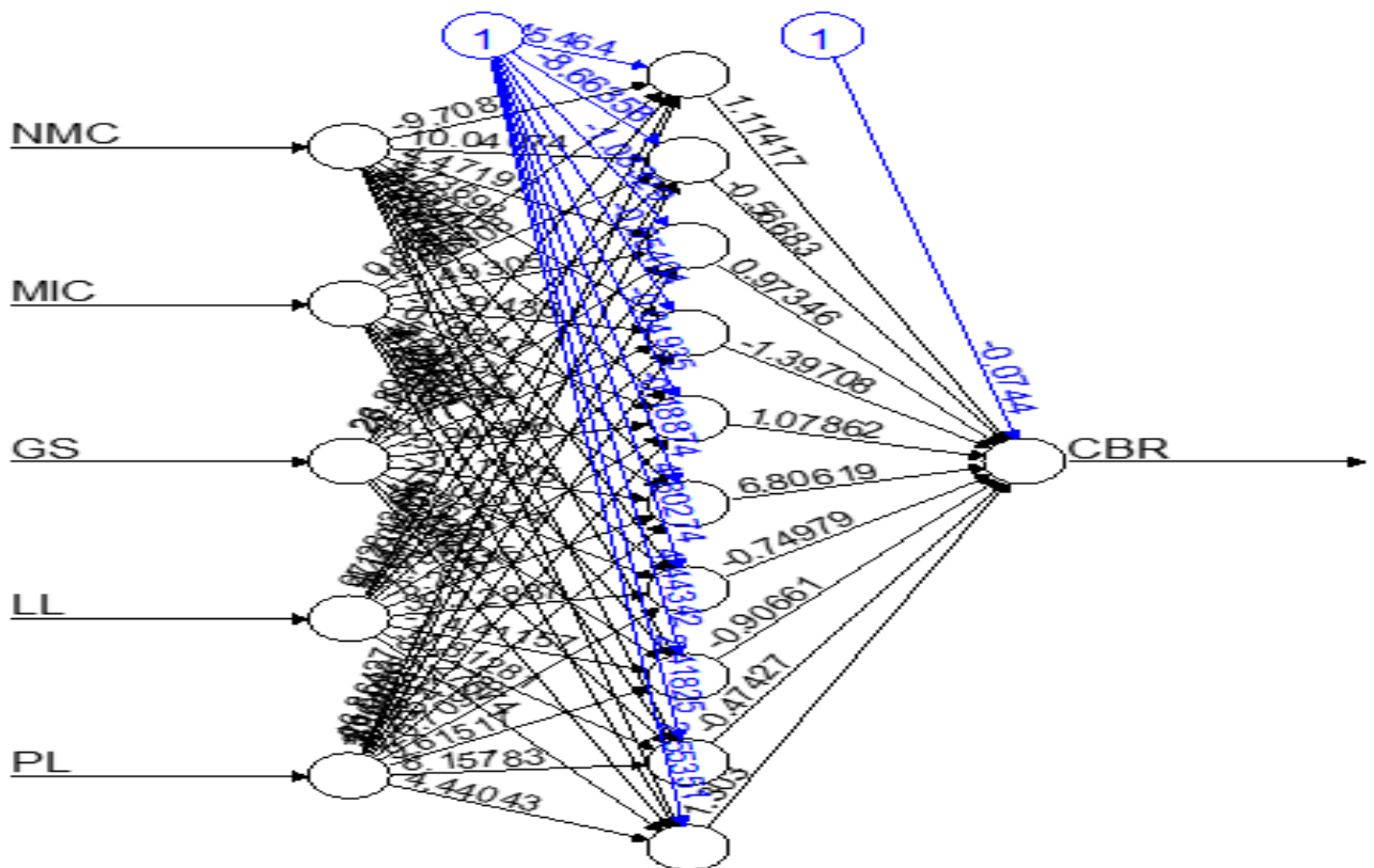
Figure 1 Neural network plot of CBR
