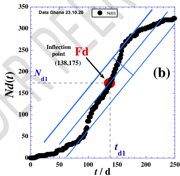
Figure 2Sb. Graphical Determination of the Inflection point F_d(t_{d1}, N_{d1}) Related the Total Death Cases N_d(t) for the first 250 days in Ghana.
