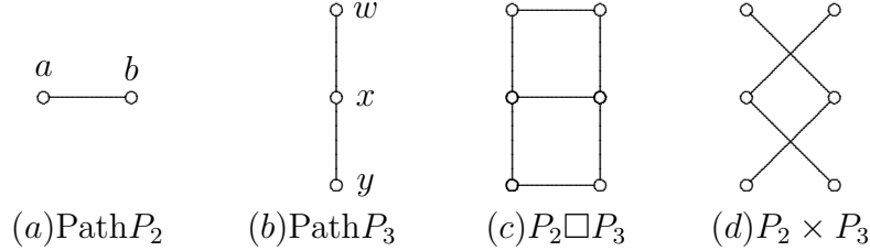
Figure 2: (a) Path P_2 (b) Path P_3 (c) Cartesian Product P_2 \square P_3 ; and (d) Direct Product P_2 \times P_3 .
