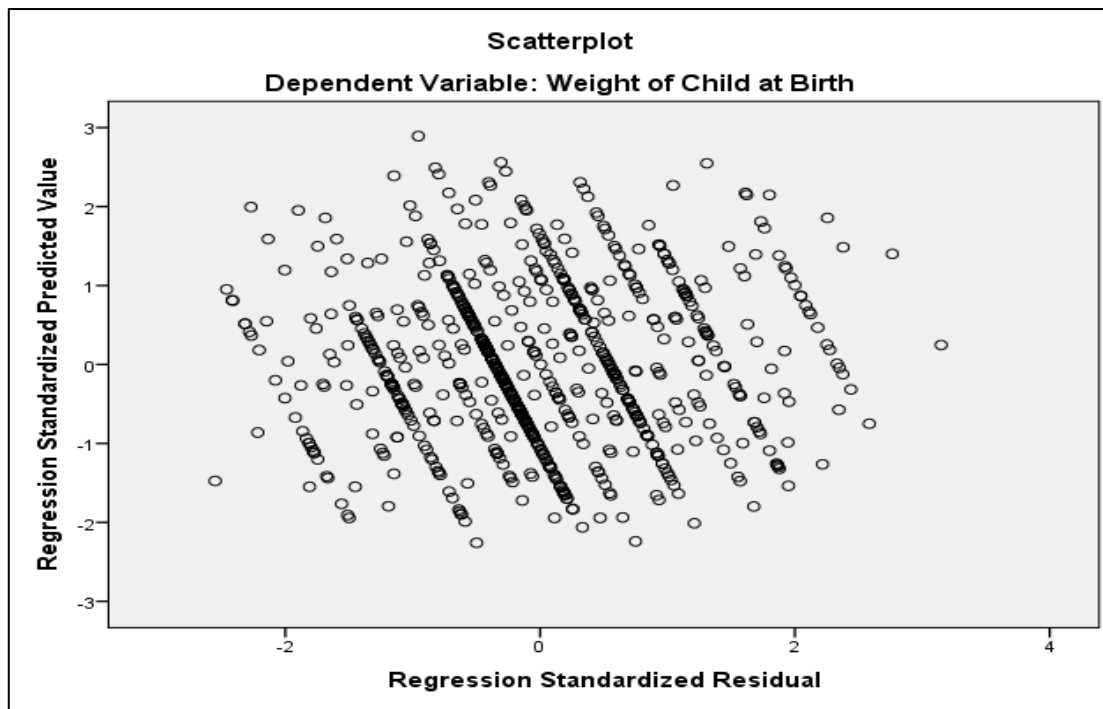
Figure 6: Constant error variance test
