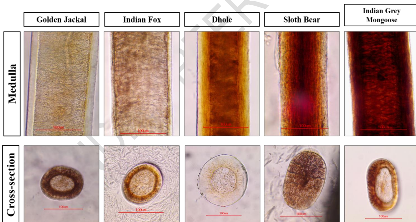
Figure 4. Medullary structures and cross-sections of hair of golden jackal, Indian fox, dhole, sloth bear and Indian grey mongoose
