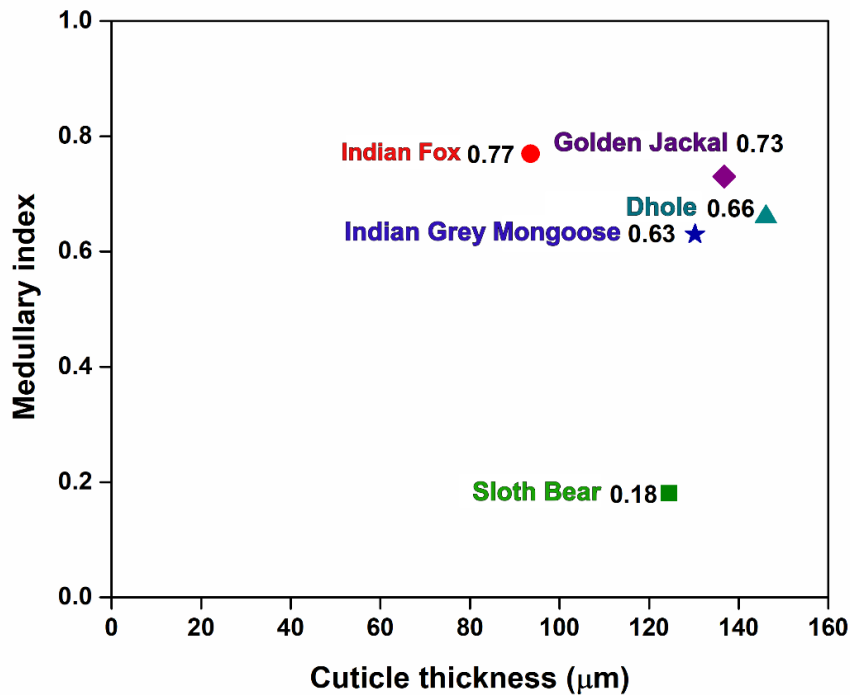
Figure 5. Cuticle thickness and medullary index of hair of carnivores. The Golden Jackal and Indian Fox can be seen at the top of the graph indicating higher medullary index but the golden jackal has comparatively thicker hair than Indian fox. The dhole and Indian grey mongoose also has similar medullary index but the difference in hair thickness shows dhole away from Indian grey mongoose. The sloth bear with its lowest medullary index is at the bottom of the graph.
