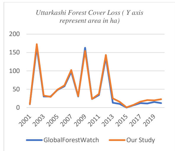
Figure 20 Plot of our study versus Global Forest Watch for Uttarkashi region.
