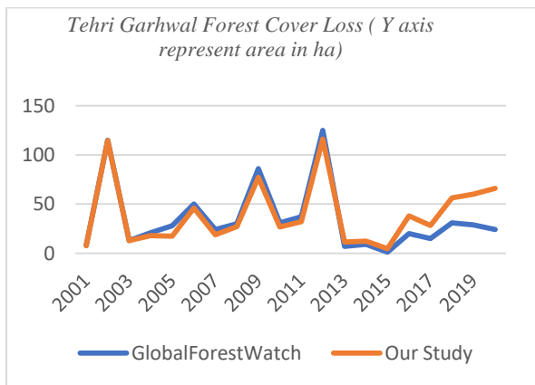
Figure 81 Plot of our study versus Global Forest Watch for Tehri Garhwal region.
