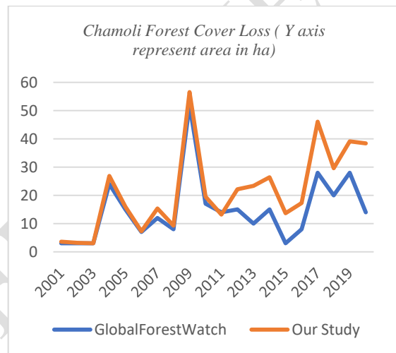
Figure 158 Plot of our study versus Global Forest Watch for Chamoli region.
