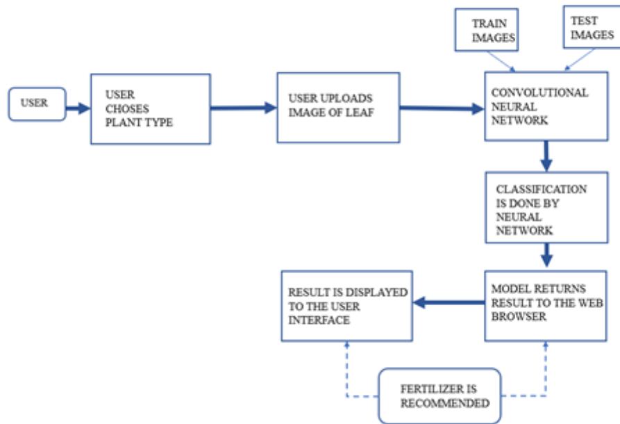
Figure 1. Proposed architecture for detecting disease on a plant leaf
