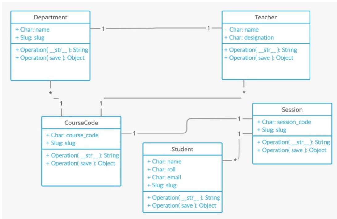
Figure 5 : Class Diagram.
