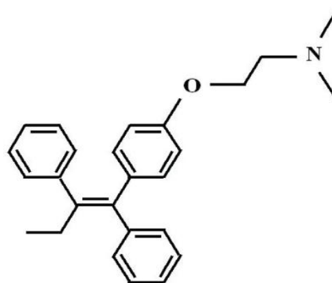
Fig. 1. Structure of tamoxifen
