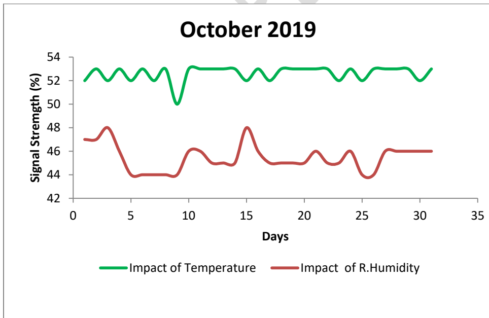
Figure 4: Comparing the effects of Temperature and Relative humidity on RSS for October 2019
