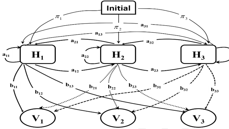
Figure 1: Schematic diagram of HMM
