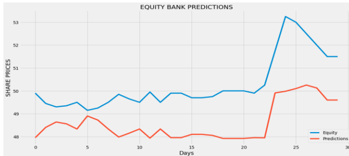
Figure 6: Equity Bank SVM Model Forecast
