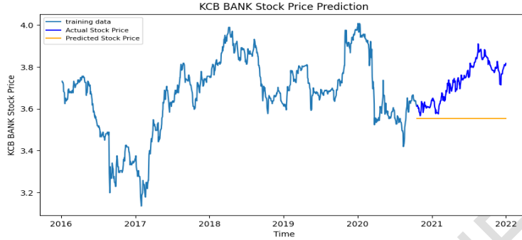
Figure 4: KCB Bank ARIMA Model Forecast
