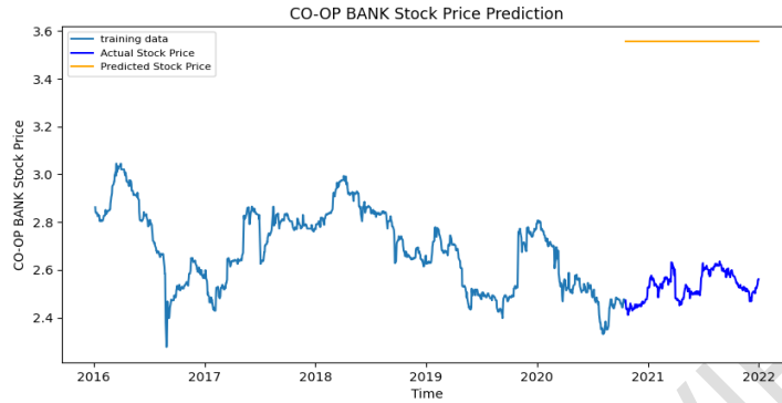
Figure 5: CO-OP Bank ARIMA Model Results
