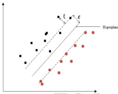
Figure 2: Set-up of a Linear SVR; Source [13].
