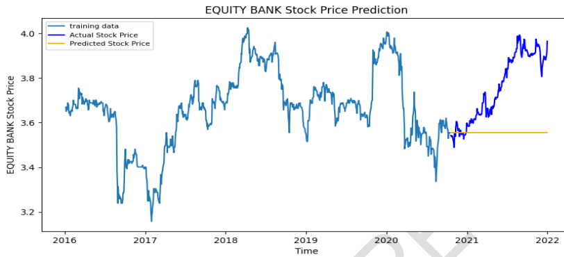
Figure 3: Equity Bank ARIMA Models Forecast
