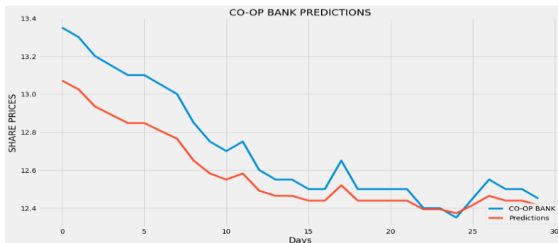
Figure 8: Cooperative Bank SVM Model Forecast
