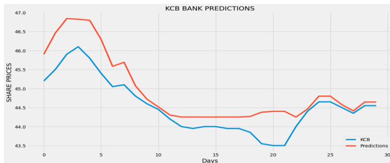
Figure 7: KCB Bank SVM Model Results
