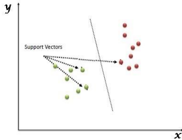
Figure 1: Support Vector Hyperplane; Source [11]
