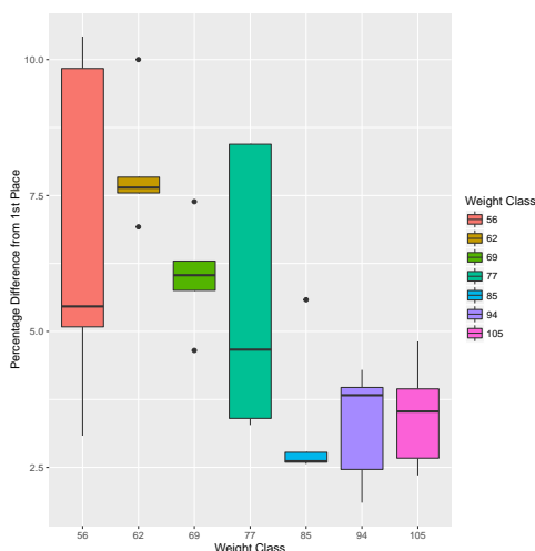
Figure 3: Percent difference of 5th place lifters from Gold medalist for male weight classes
