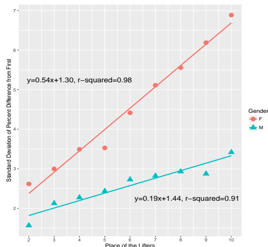
Figure 2: Standard deviation of the percent difference from first as the place a lifter attains changes
