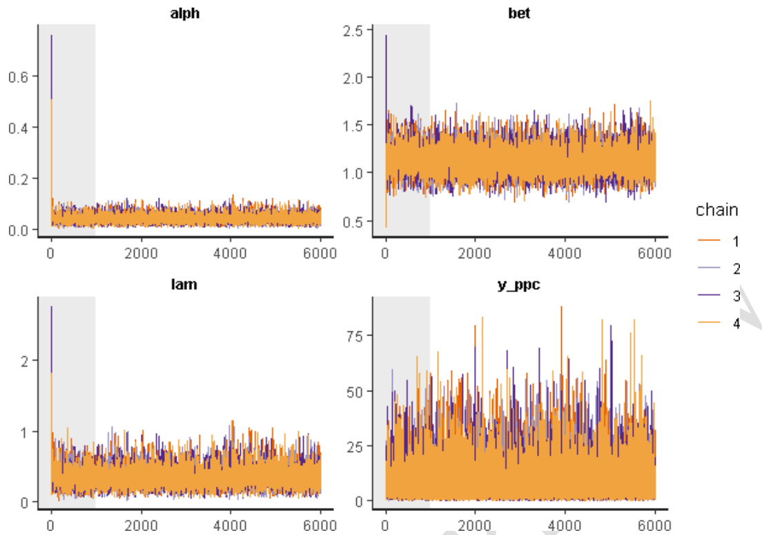
Figure 2: Traceplot of the 4 chains sampled from the posterior distribution of the parameters and the data (Remission Times)
