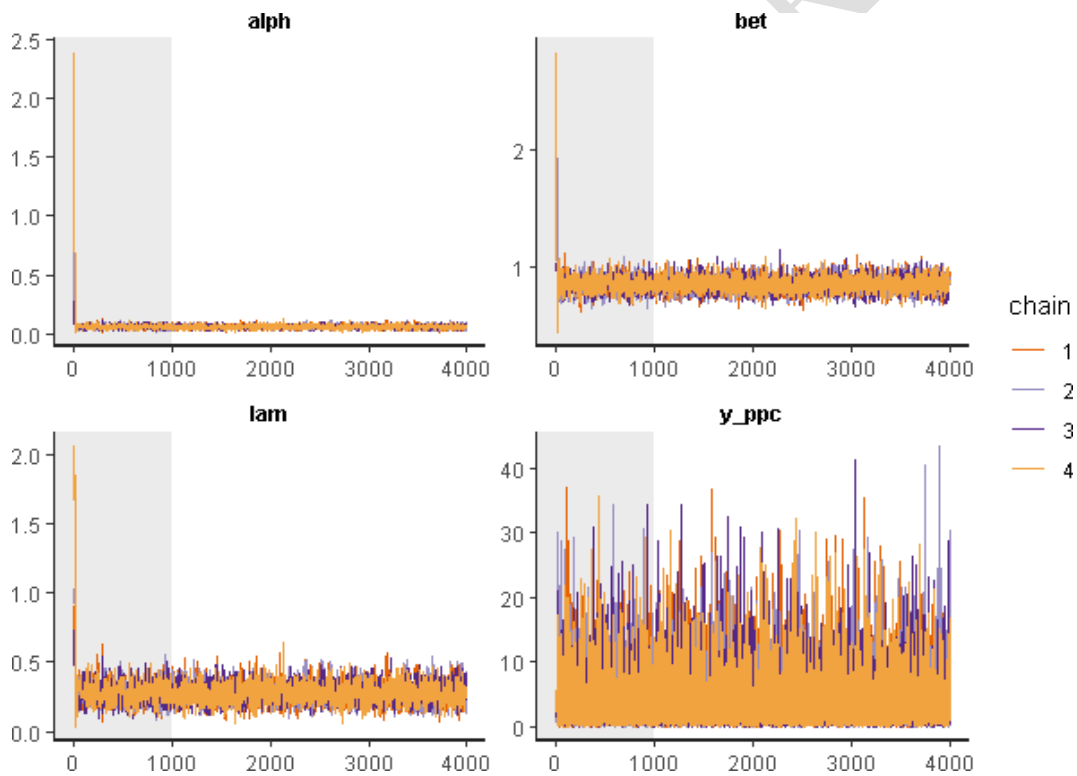
Figure 5: Traceplot of the 4 chains sampled from the posterior distribution of the parameters and the data (COVID-19 Survey in Andalusia)
