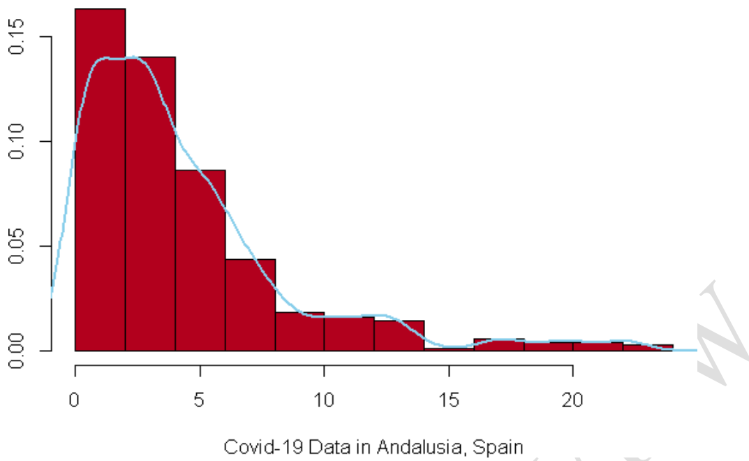
Figure 4: Histogram of COVID-19 Survey in Andalusia, Spain
