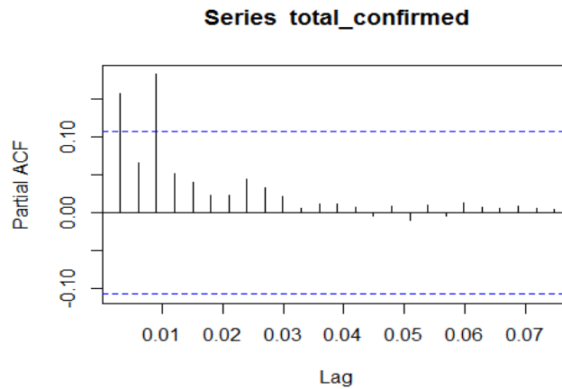
Fig. 3. Partial Autocorrelation Function (PACF) of the differenced total confirmed cases Lag one to lag four are the most significant but for convenience, AR(1) and AR(3) terms were suggested
