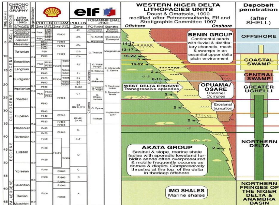
Figure 5: Regional Stratigraphy of Western Niger Delta (Reijers, 2011).
