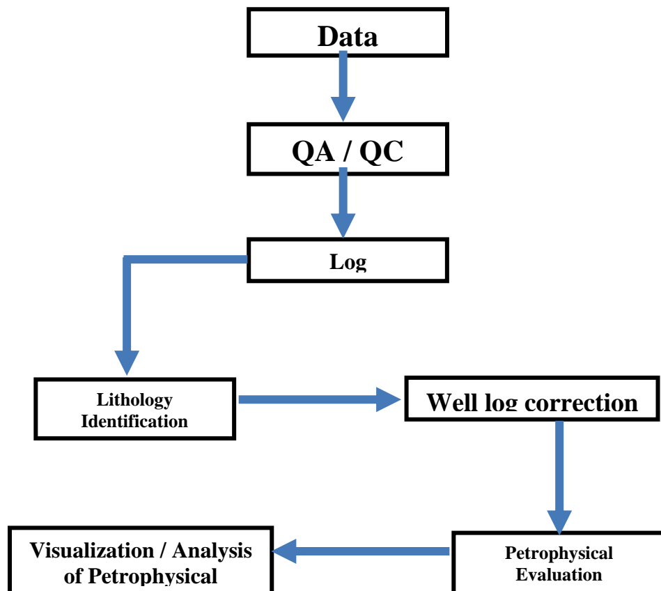
Fig. 6: Schematic of the Workflow for the Reservoir Study of BAK Field.
