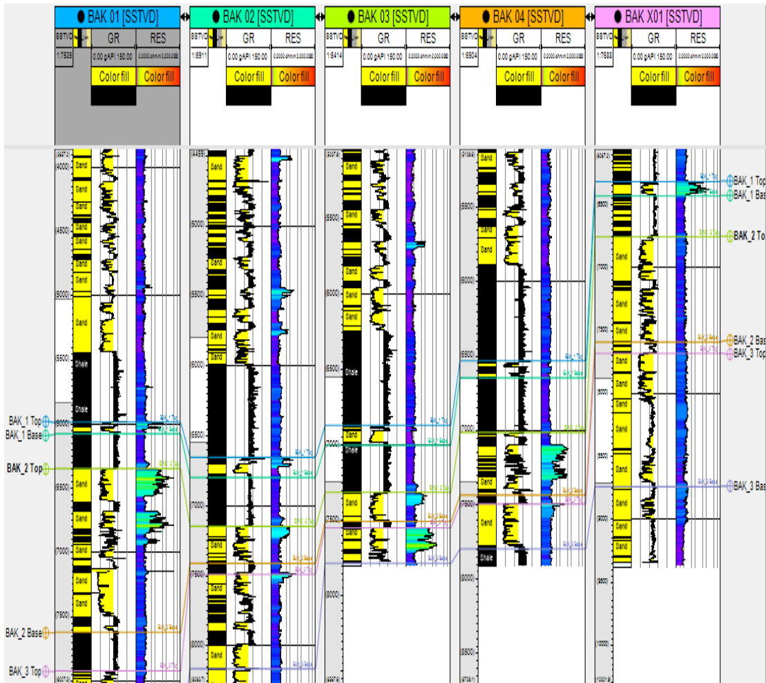
Fig. 7: Lithostratigraphic Correlation of the Five wells in BAK field showing three reservoir sand units.
