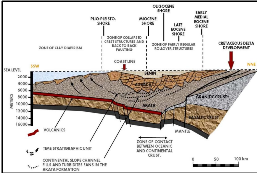
Fig. 3: Schematic dip section of the Niger Delta (Modified from Weber and Daukoru, 1975)
