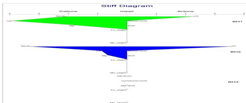
Figure 6: Stiff diagram
