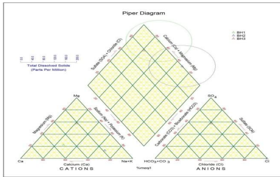
Figure 4: Piper diagram
