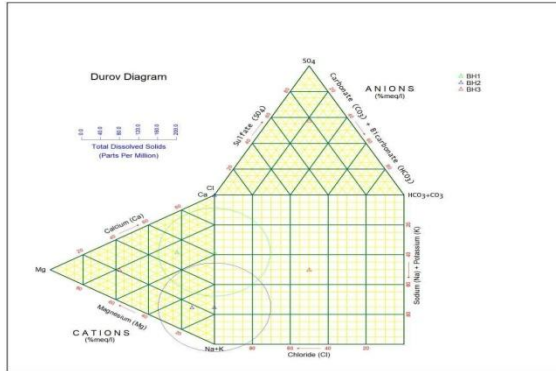
Figure 5: Durov diagram
