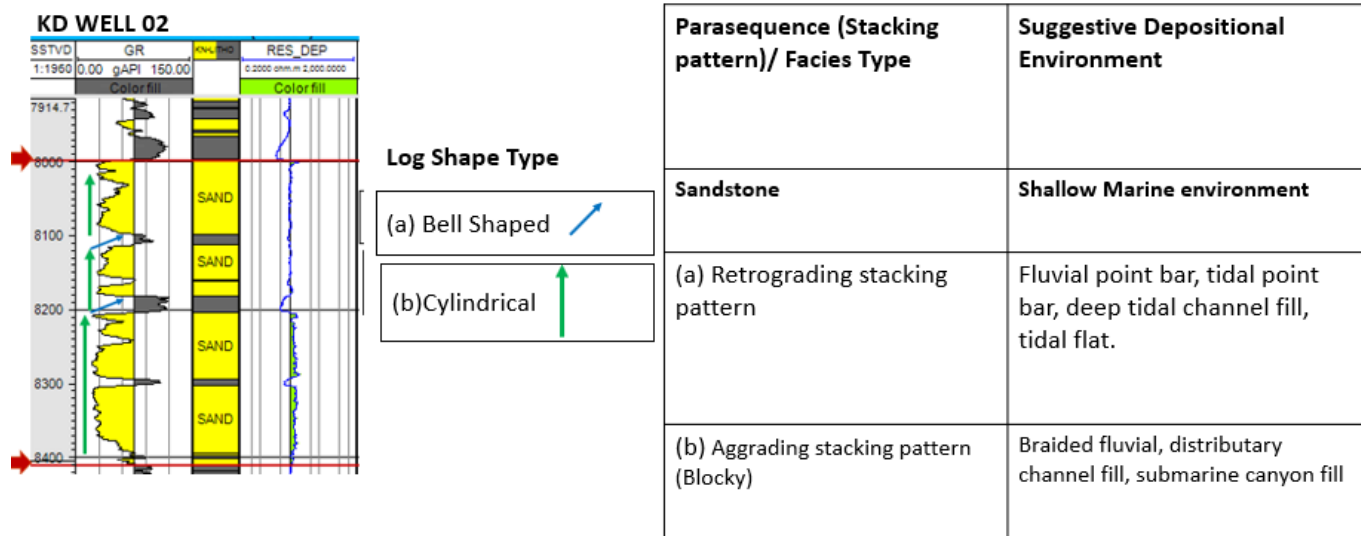
Figure 5: Parasequence and Delineation of Environment of deposition using Log Motif for KD 02 well (Reservoir-A)
