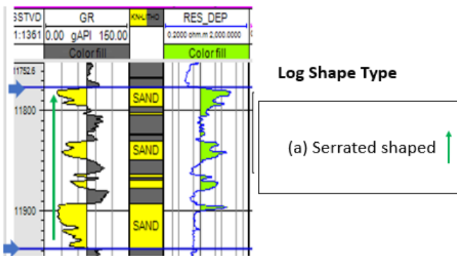
Figure 8: Parasequence and Delineation of Environment of deposition using Log Motif for KD 03 well (Reservoir-C)
