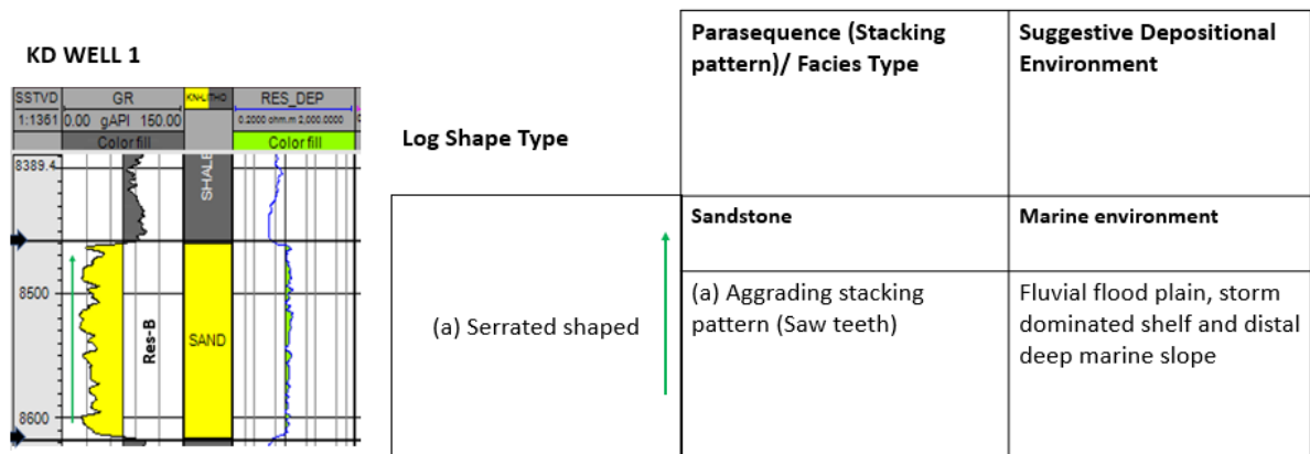
Figure 3: Parasequence and delineation of environment of deposition using log motif for KD 01 well (Reservoir B)
