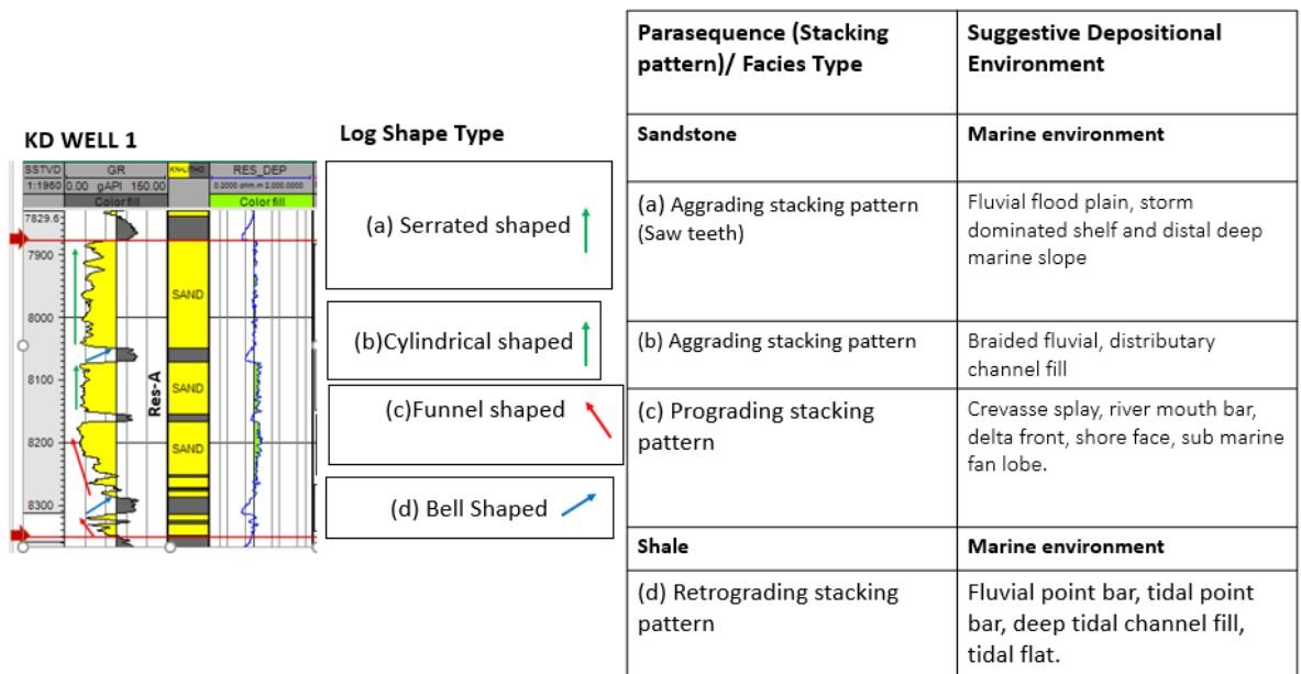
Figure 2: Parasequence and environment of deposition using Log Motif of KD 01 well (Reservoir A) After [20]
