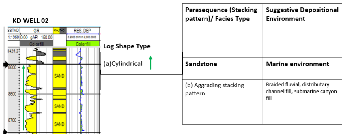
Figure 6: Parasequence and Delineation of Environment of deposition using Log Motif for KD 02 well (Reservoir-B)
