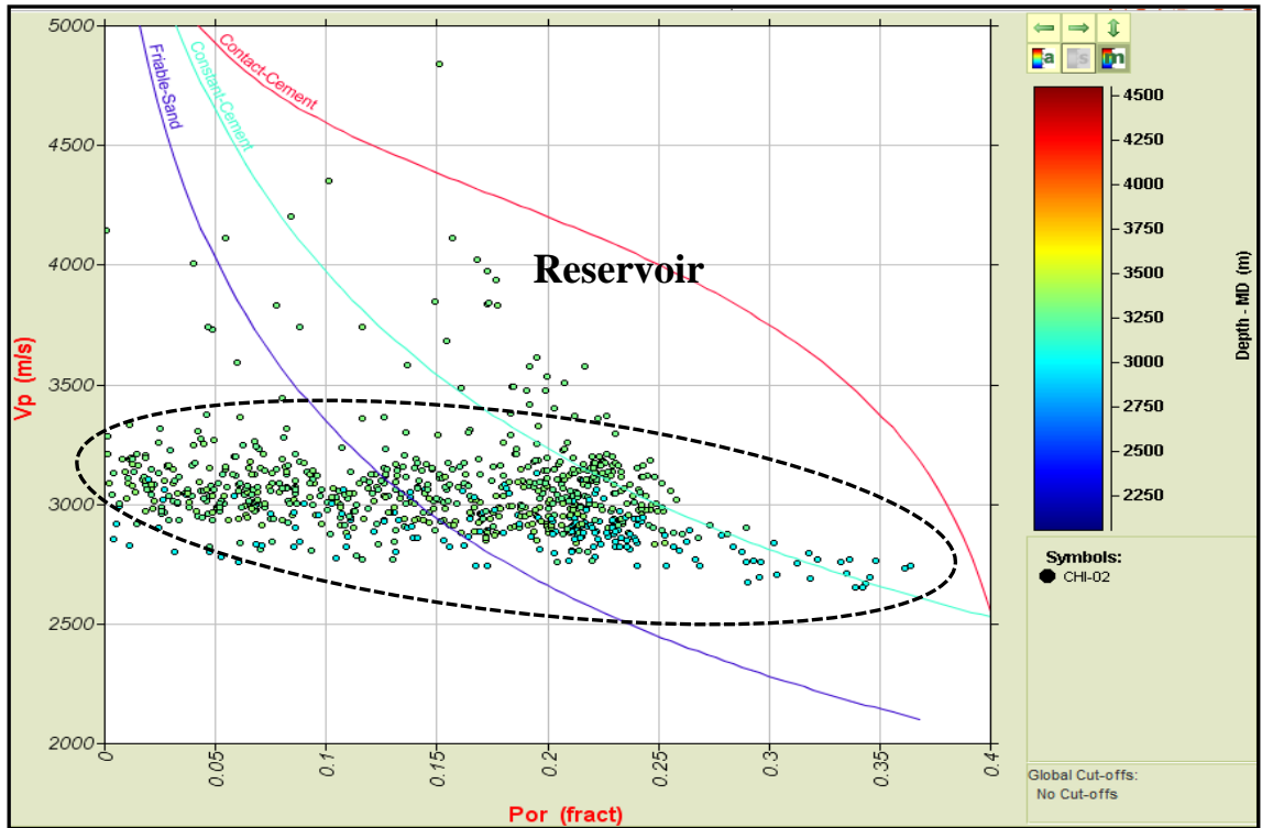
Fig. 6: Cross-plots of Velocity against Porosity Color-coded at reservoir interval with Depth for CHI-02 Well
