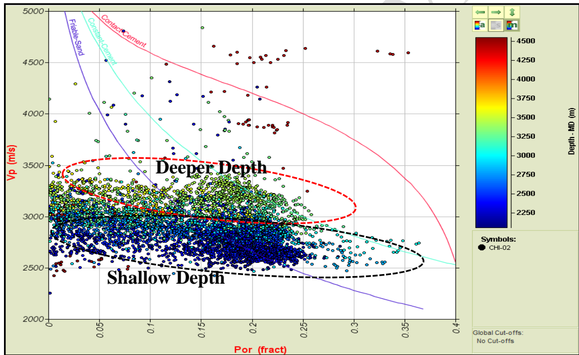
Fig. 5: Cross plots of Velocity against Porosity Color-coded with Depth for CHI-02 well
