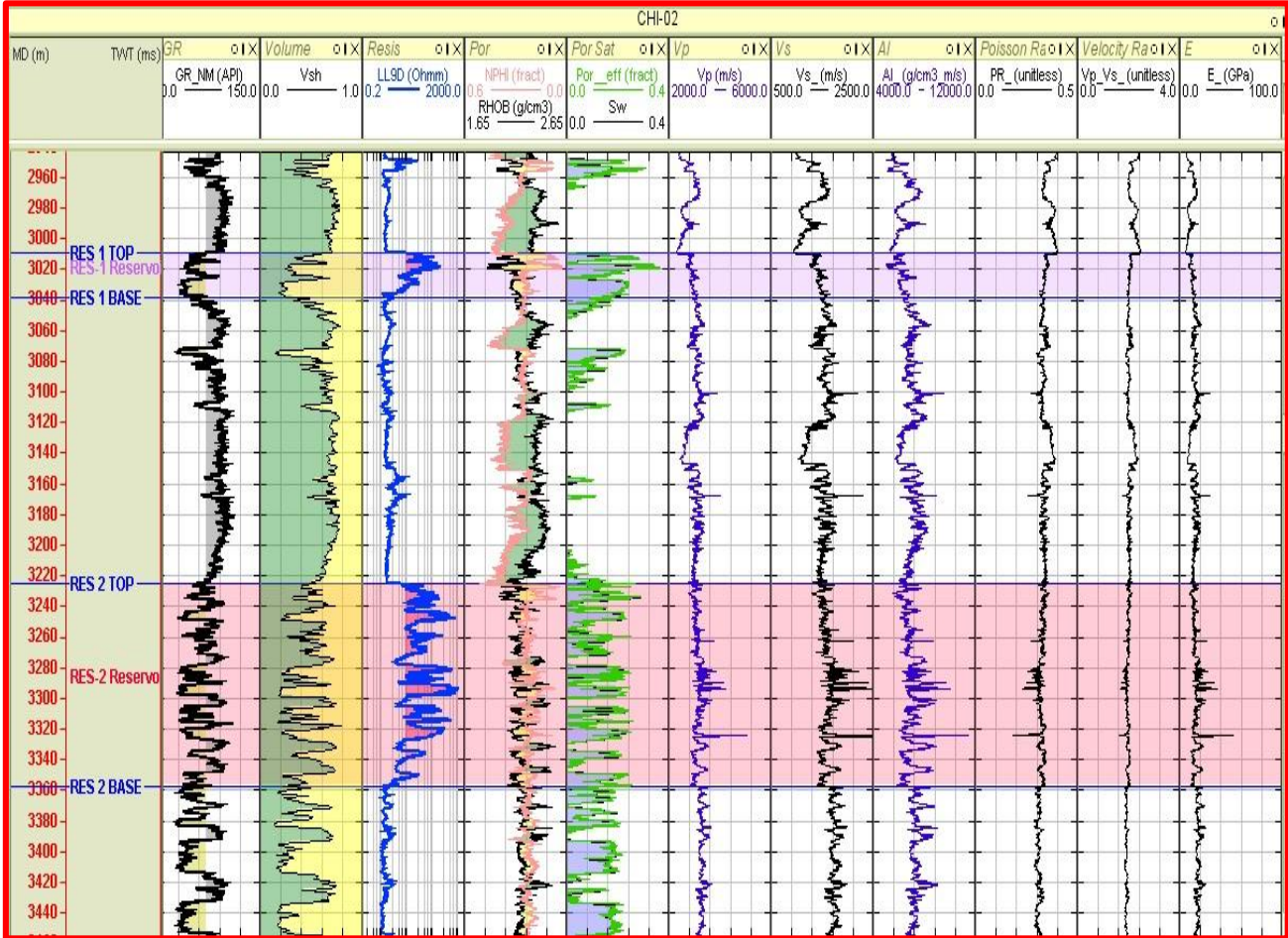
Fig. 8: Log Plots of Elastic and Reservoir Parameters Generated for CHI-02 Well
