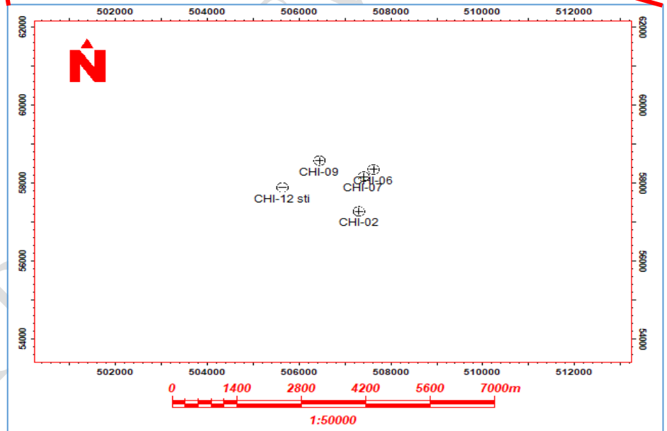
Fig.1: Location and the base map of the study area
