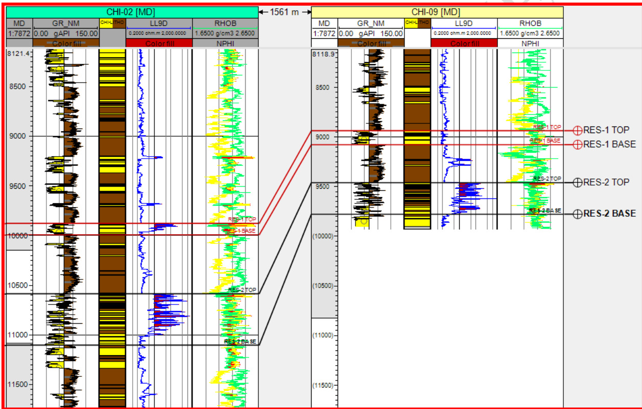
Fig 3: Lithostratigraphic Correlation of CHI Well 02 and 09
