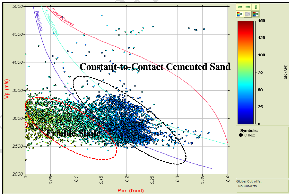
Fig. 4: Cross plots of Velocity against Porosity Color-coded with gamma ray for CHI-02 well
