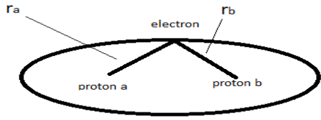
Fig.2a The Hydrogen Molecular Ion.
