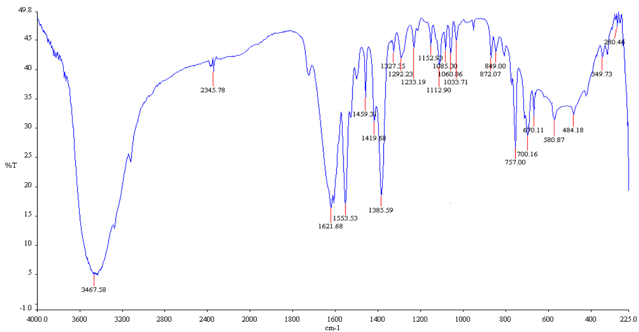
Figure 4: IR spectrum of NiL1
