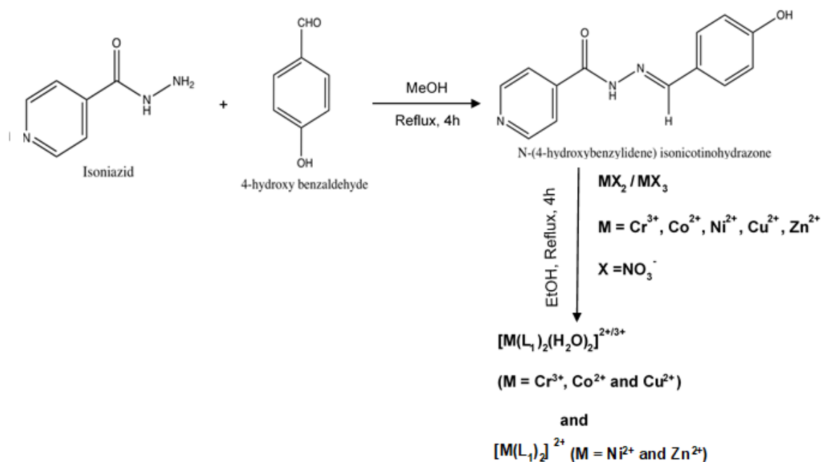
Scheme 1: Synthesis of the Schiff base ligand, L1 and its metal complexes
