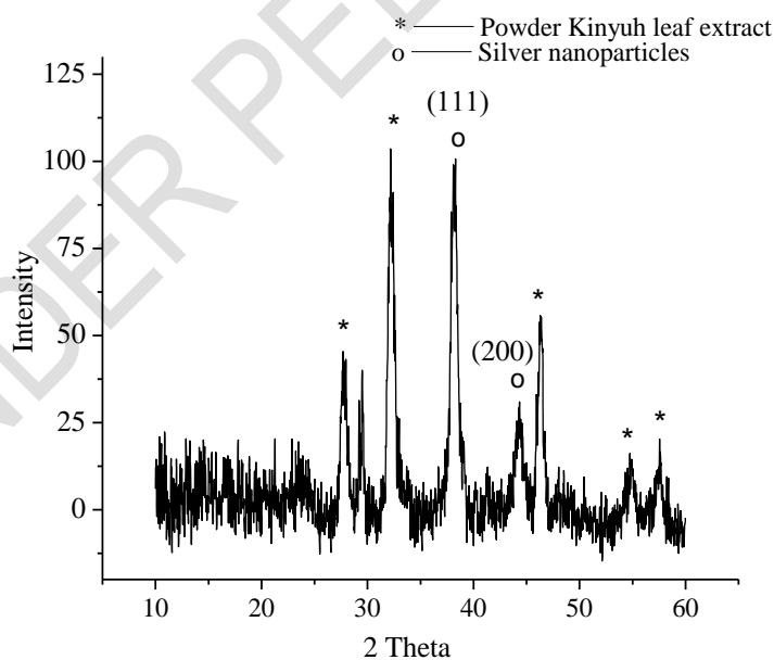
Fig 3. XRD pattern of silver nanoparticles
