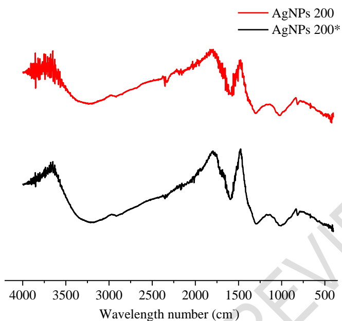
Fig 4. The FTIR Spectra of silver nanoparticles
