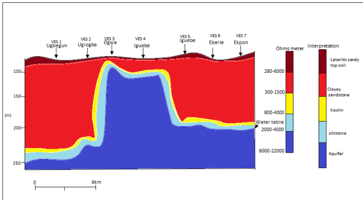
Fig. 7: Geo-electrical resistivity section of the study area
