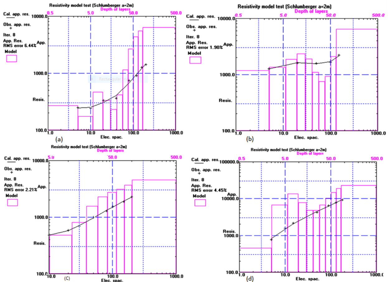
Fig. 5: (a) Inverted model layer for VES 1 taken at Ugbejun (b) Inverted model layer for VES 2 taken at Ugiogba (c) Inverted model layer for VES 3 taken at Ogwa (d) Inverted model layer for VES 4 taken at Iguebe north in Edo State
