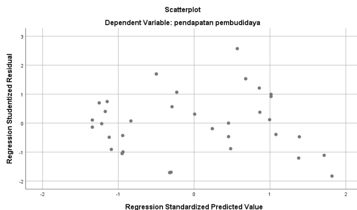
Fig 2. Heteroscedasticity
