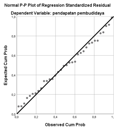
Fig 1. Normality Test
