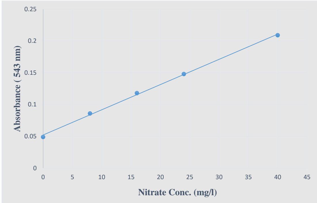
Figure 4. Standard curve of \text{NO}_3^- , and correlation equation Y=0.05228 + (0.00396) X ; where Y is Absorbance, and X is Nitrate concentration (mg/l). This equation permits to calculate nitrate concentrations in the mini-pond during experimental time.
