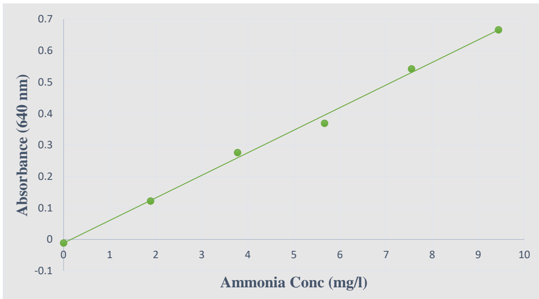
Figure 3. Standard curve of (\text{NH}_3, \text{NH}_4^+) and correlation equation Y=-0.0112+ (0.0717) X ; where Y is Absorbance, and X is Ammonia concentration (mg/l). This equation permits to calculate ammonia concentrations in the mini-pond during experimental time.
