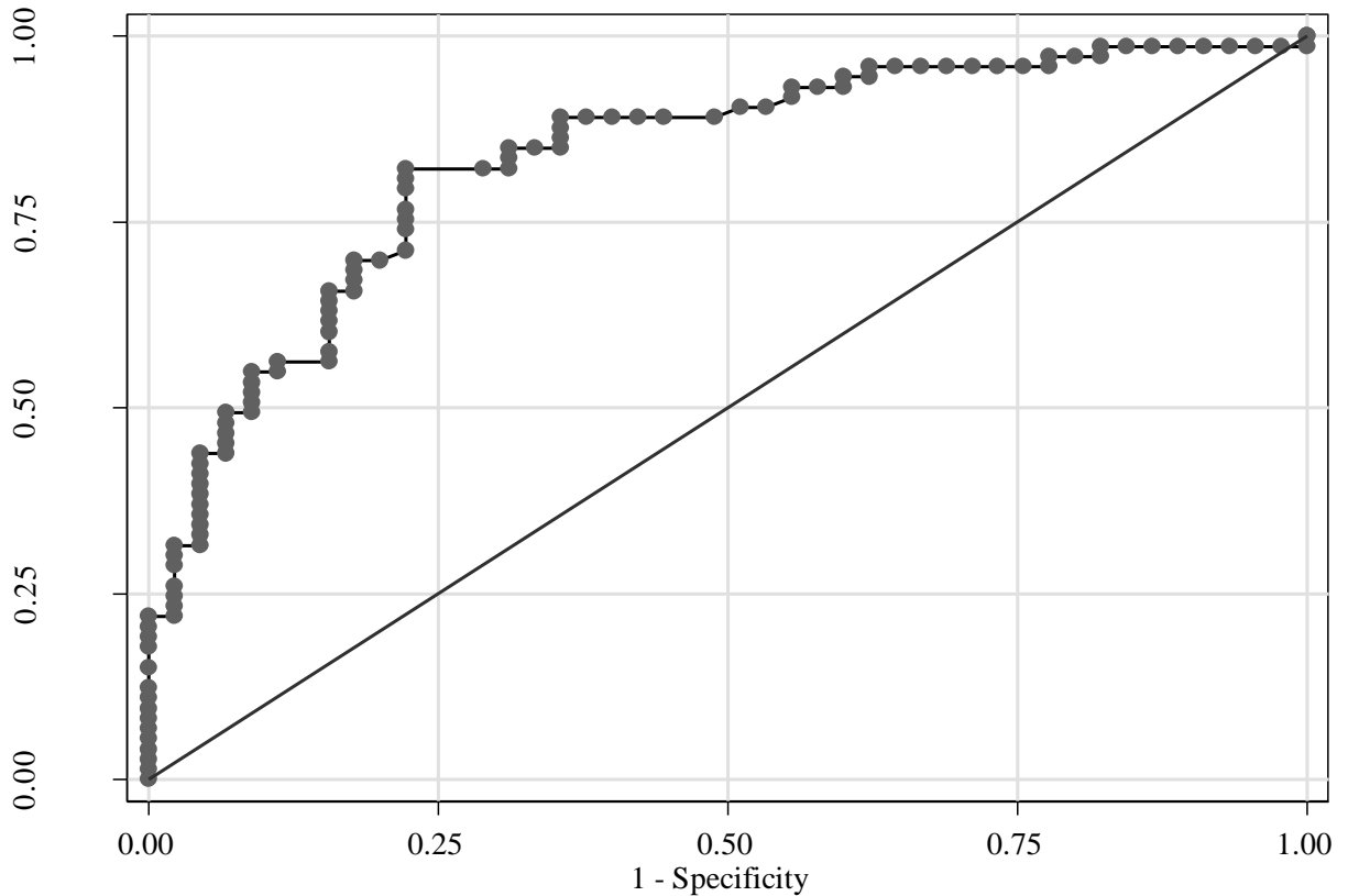
Figure 2:ROC Curve
