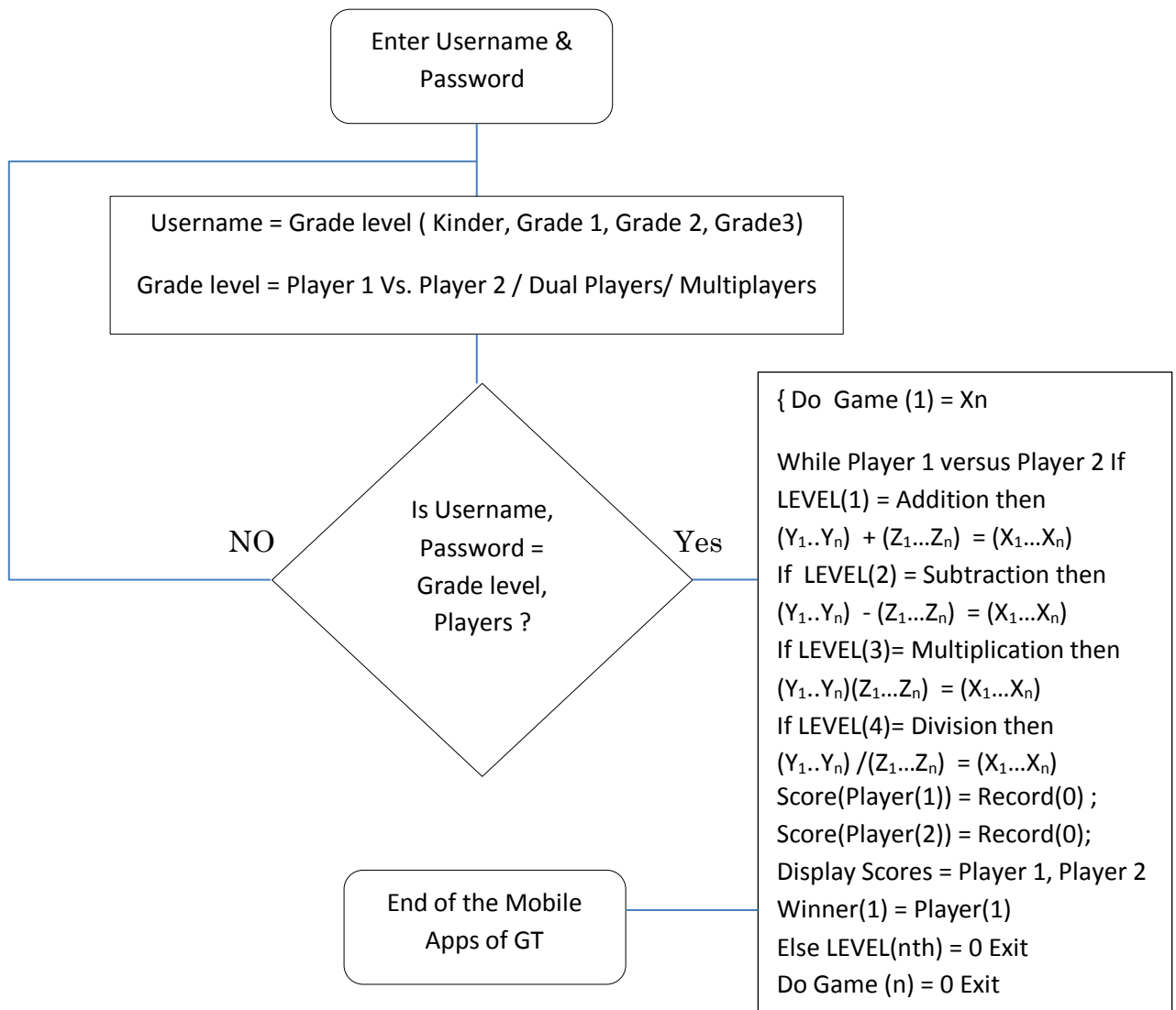
FLOWCHART 1. The SAD (System Analysis Design) of the Proposed Mobile apps of GBL
