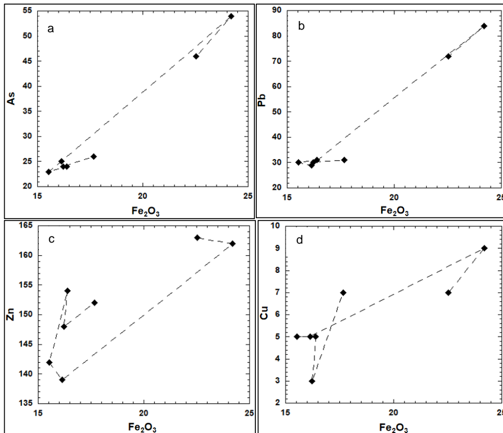
Figure. 4 a-d Correlations between Fe_2O_3 and As, Pb, Zn and Cu.
