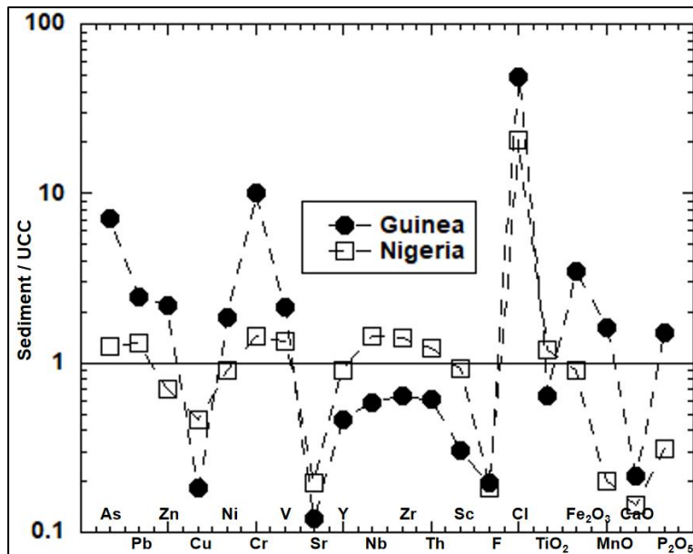
Figure 3. Comparison of trace and major element concentration in surface sediments of Guinea and Nigeria mangrove. All values were normalized to the UCC values of [15].
