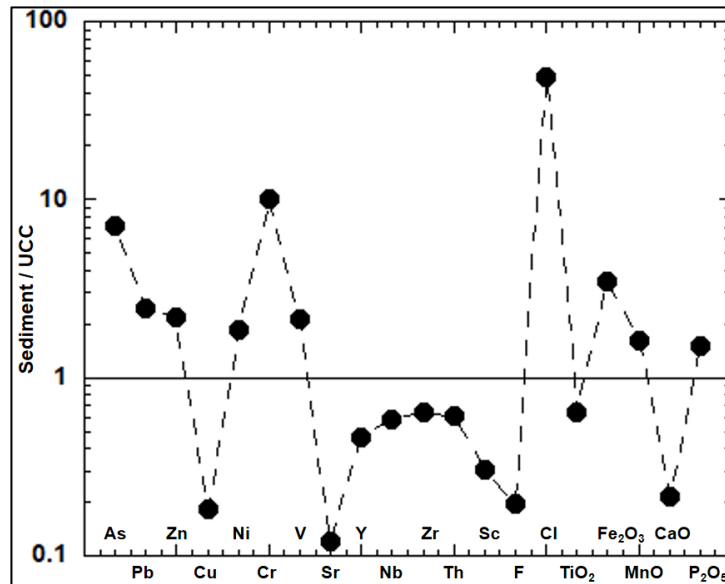
Figure 2. Comparison of trace and major element concentration in surface sediments of Conakry mangrove. All values were normalized to the UCC values of [15].
