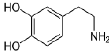
C. Dopamine molecular Structure
