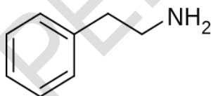
B. Phenylamine Structure
