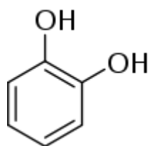
A. Catechol structure
