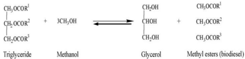
Figure 1: Transesterification in biofuel production.
