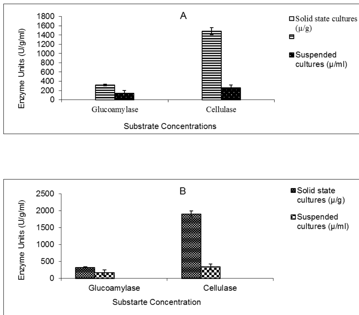
Fig 5: Comparison of enzyme production by Fusarium sp (A) and Rhizopus sp (B) in solid state and suspended cultures
