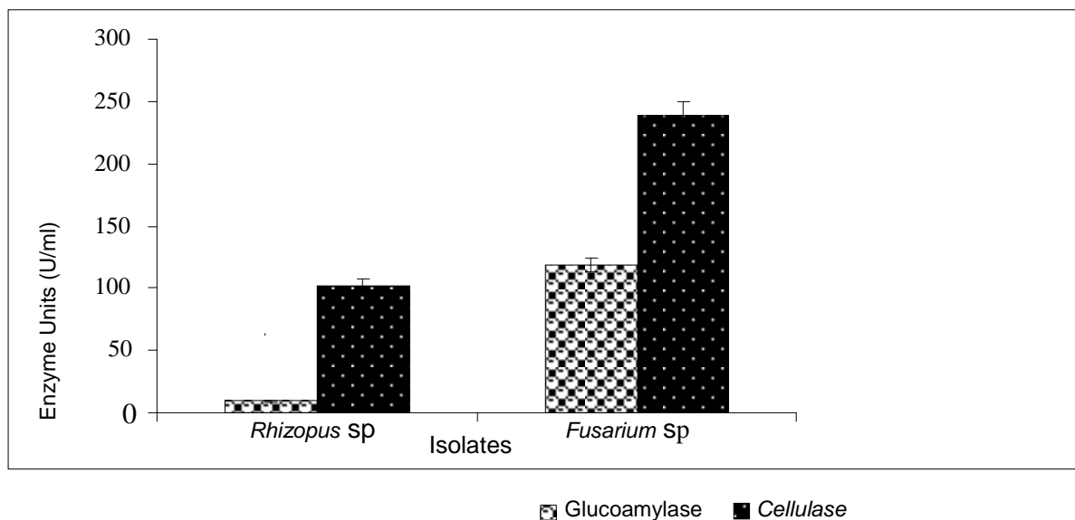
Figure 1: Screening of the isolates for the production of both glucoamylase and cellulase enzymes in suspended culture
