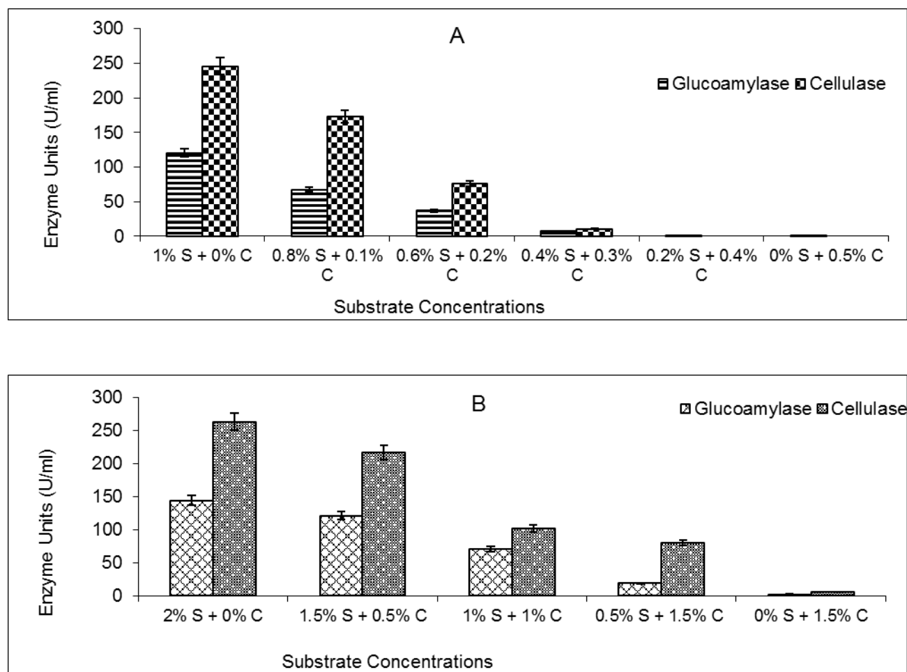
Fig 3: Effect of ratios of starch to cellulose on enzyme production by Fusarium sp.
