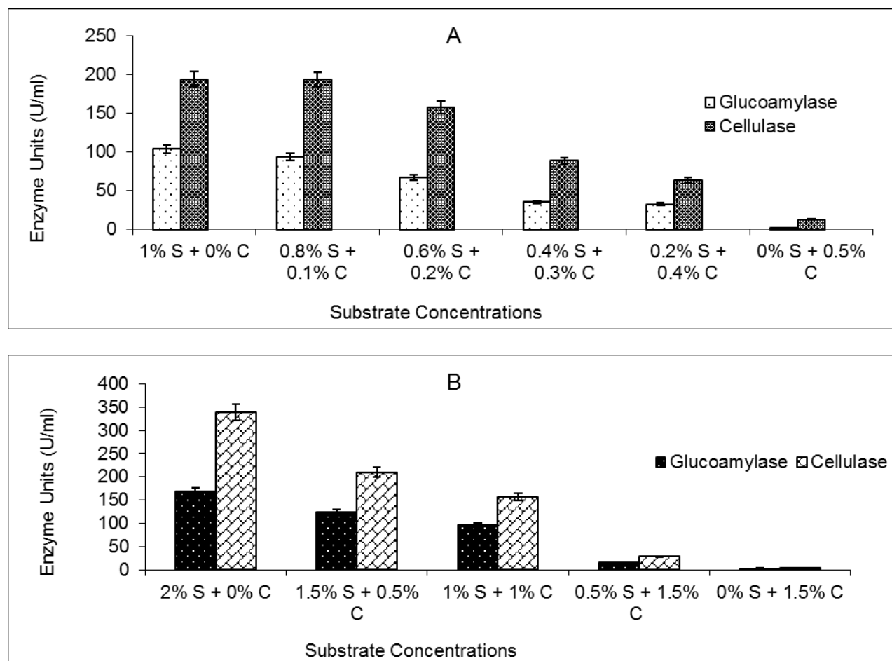
Figure 2: Effect of the ratios of starch to cellulose on enzyme production by Rhizopus sp.
