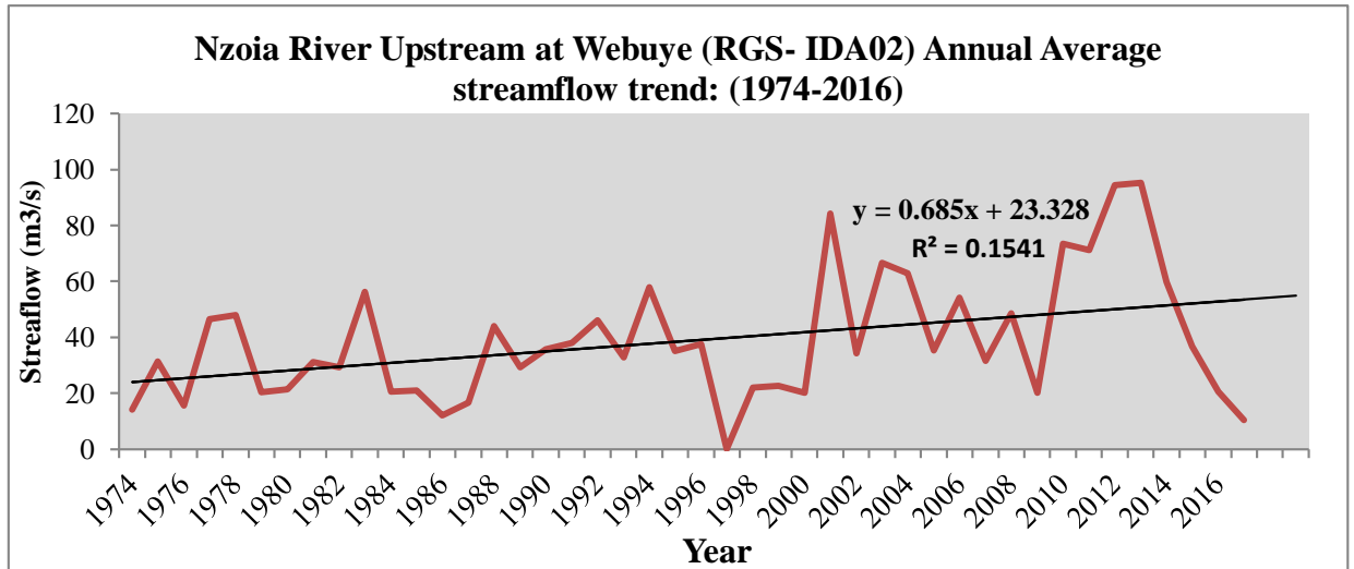
Figure 14: Annual stream flow trend for Nzoia river upstream at Webuye (IDD01)
