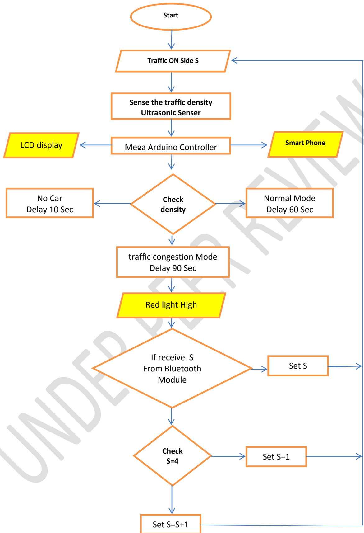
Fig.6 . Flow chart of the system
